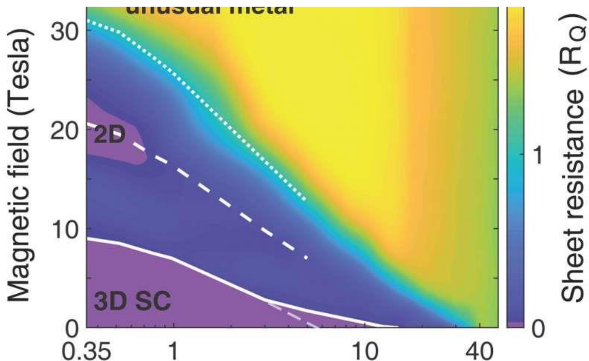
A phase diagram of LBCO at different temperatures and magnetic field strengths. Colors represent how resistant the material is to the flow of electrical current, with purple being a superconductor with no resistance. When cooled to near absolute zero with no magnetic field, the material acts as a 3-D superconductor. As the magnetic field strength goes up, 3-D superconductivity disappears, but 2-D superconductivity reappears at higher field strength, then disappears again. At the highest
