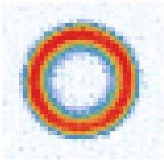
Photo of a BEC in a ring-shaped matterwave
