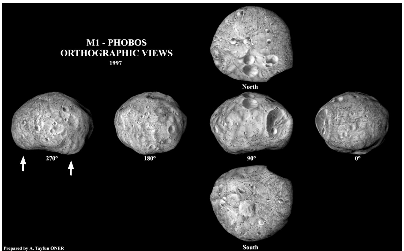
Fig.16. The Phobos' picture produced by A.Tayfun Oner shows six different orientations. The images were rendered by using Peter C. Thomas model and USGS airbus map of the satellite. Middle row: 0^\circ - Sub-Mars hemisphere, 90^\circ - Leading hemisphere, 180^\circ - Anti-Mars hemisphere, 270^\circ - Trailing hemisphere. Phobos' longer axis is directed towards its parent body as is the case for most bodies in the solar system. The remnants of original cone apex separated owing to plastic evolution are pointed by white arrows. ( http://solarviews.com/cap/mars/phobos6.htm )
