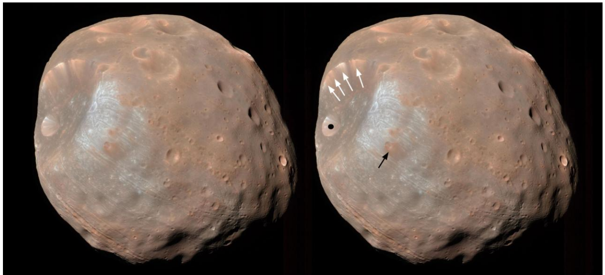
Fig.21. Left: Phobos with Stickney crater imaged by Mars Reconnaissance orbiter on 23 March 2008. Colors combine data from camera's blue-green, red, near-infrared channels. Artificial color data accentuate details of red and blue spectral units. Right: Locations of brighter streaks on Stickney slopes are marked with arrows. Crater Limtoc with similar streaks inside is black dotted. Black arrow points to fresh red unit ejecta of a newly formed crater inside big blue unit area. ( http://photojournal.jpl.nasa.gov/catalog/PIA10368 )
