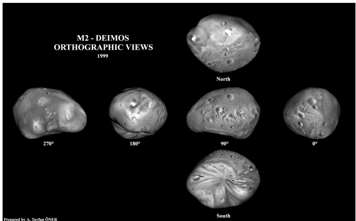
Fig.11. The Deimos' picture (by A.Tayfun Oner) shows six different orientations. The images were rendered by using .P.C. Thomas model and a combination of the USGS map and Deimos' photomosaic. 0° - Sub-Mars hemisphere, 90° - Leading hemisphere, 180° - Anti-Mars hemisphere, 270° - Trailing hemisphere. ( http://solarviews.com/cap/mars/deimos6.htm )
