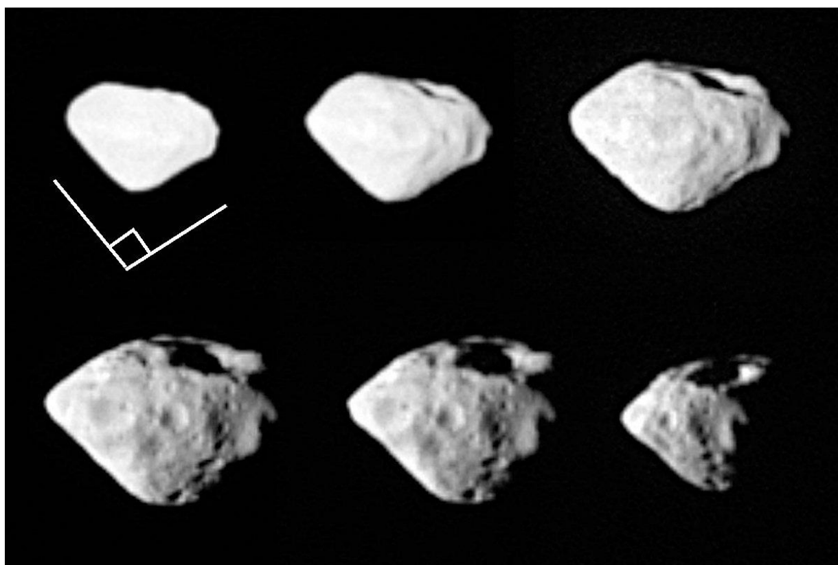
Fig.1. Six views of approx two thirds of Steins' surface acquired by OSIRIS imaging system before, during, and after the close encounter. White sketch was added by us to emphasize ca. 90^\circ northern pole summit angle.
