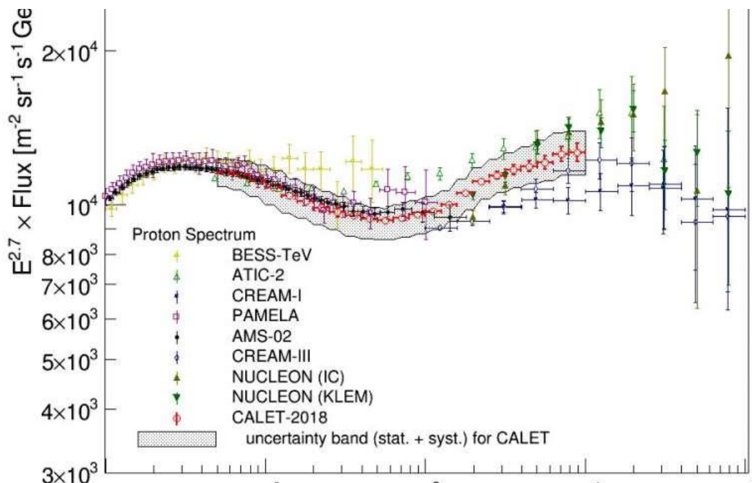
Cosmic-ray proton spectrum measured by CALET (red points) from 50~GeV to 10~TeV, together with recent direct measurements. Credit: Adriani et al.
