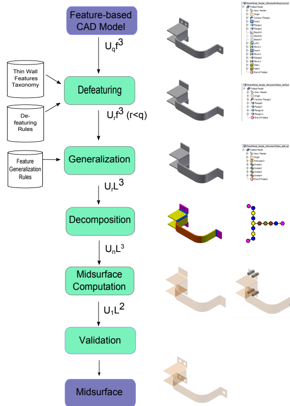
Figure 2: Overall work-flow
