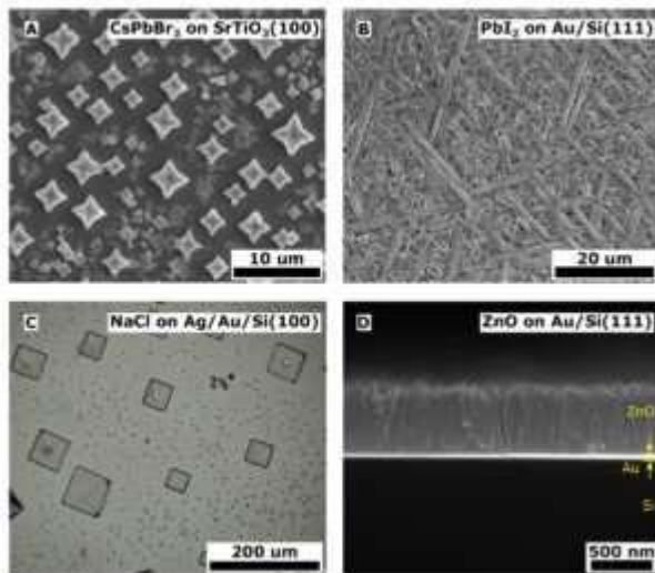
Electron and optical microscope images of epitaxial (A) cesium lead bromide, (B) lead iodide, (C) sodium chloride and (D) zinc oxide. Credit: Science 2019
