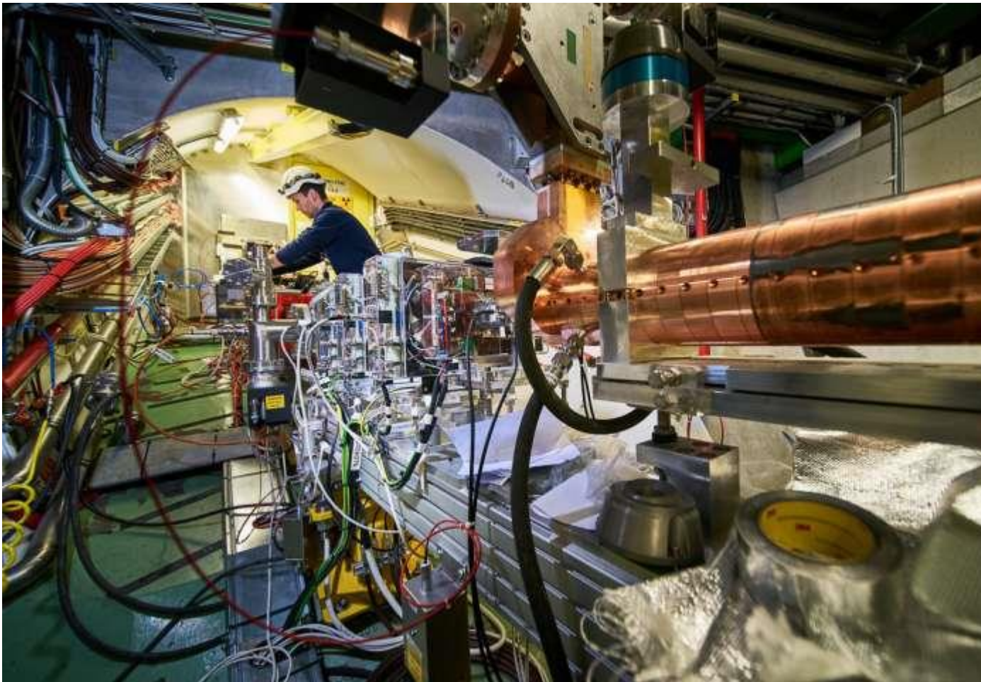
The AWAKE experiment uses a proton beam to create a strong plasma wakefield. Credit: CERN
