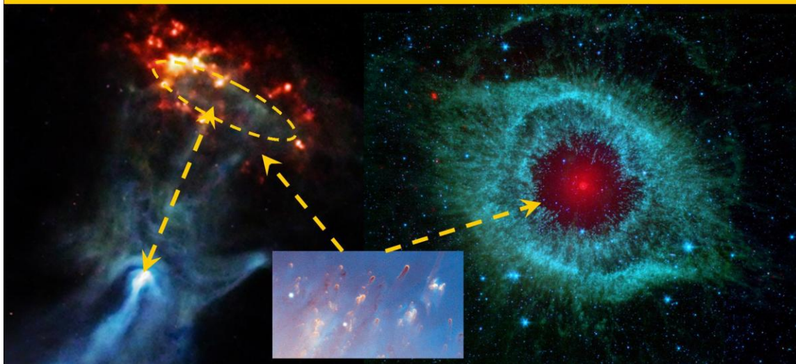
Figure 10, The A-symmetric B 1509-58 nebula , and symmetric Helix nebula as examples of the difference between Fermion and Black hole Quantum Gravity effects.
