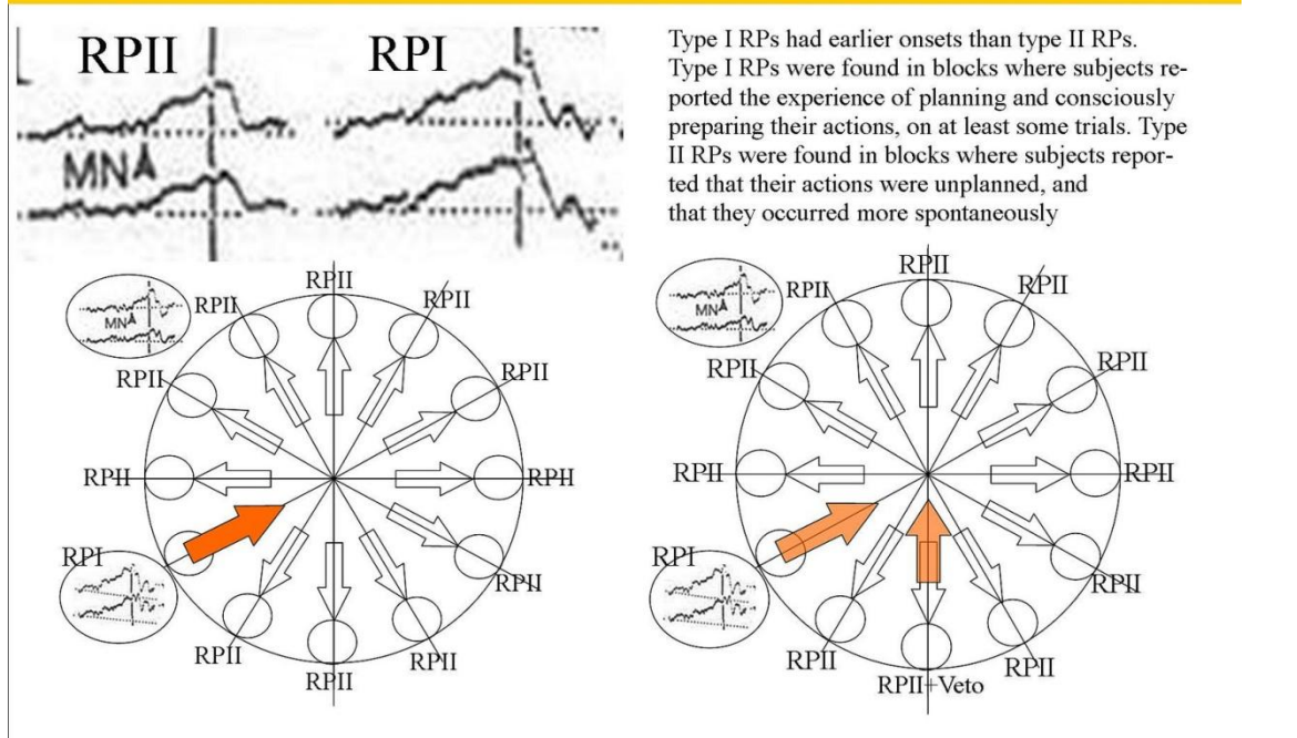
Figure 32, Quantum FFF Theory explanation of the difference between RPI and RPII ( R=Readiness potential) observed and published by Benjamin Libet around 1964. ( reference: 72: Democratic Free Will and Telepathy in the Instant Entangled Multiverse )
