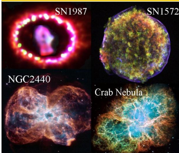
Figure 11, Other examples of Quantum Gravity effects on ejected rings of micro black hole starspots at work in different nebula .
