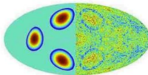
Figure 2, wavefunction collapse between CP symmetric mirror particles by instant entanglement between multi universal bubbles located around the Big Bang central void.
