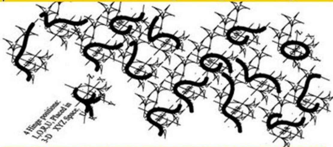
Figure 34, Sterile Neutrinos and Majoranas seem to have a different origin.
