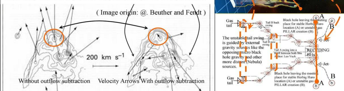
Figure 35. Example of NGC 326: The Repelling of Two Equal sized Black Holes as the formation of a Herbig Haro Bowshock system, with star formation in between and double jets. According to Quantum FFF Theory.
