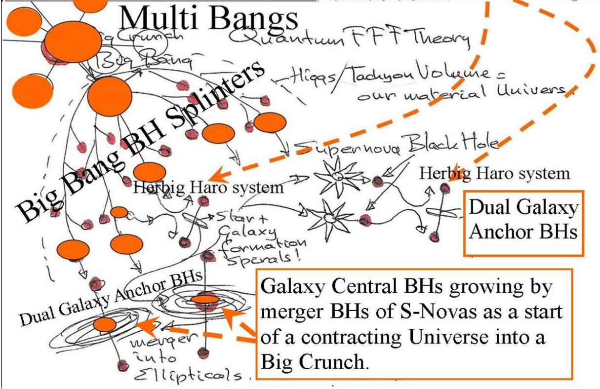
Figure 18, The Cyclic Multiverse.
