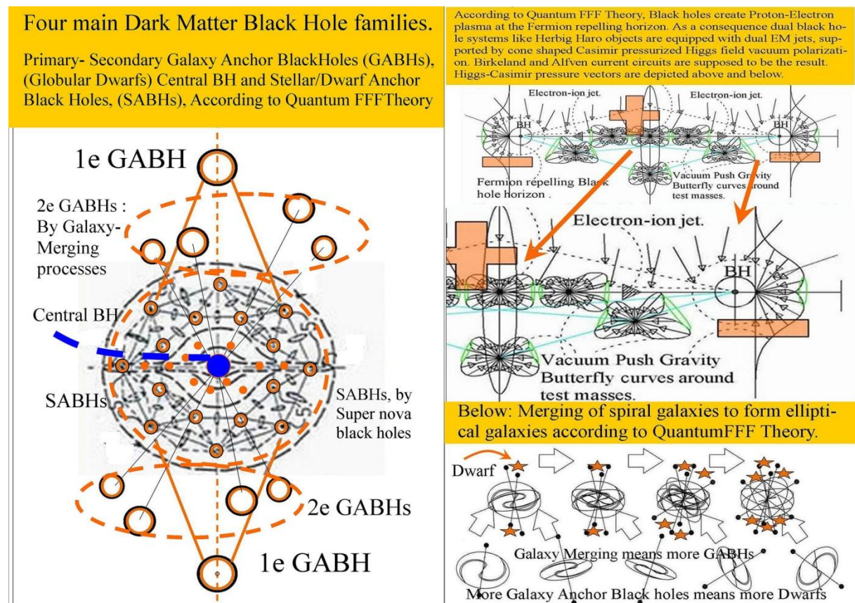
Figure 15, GABHs as the largest unit of Dark Matter black hole families
