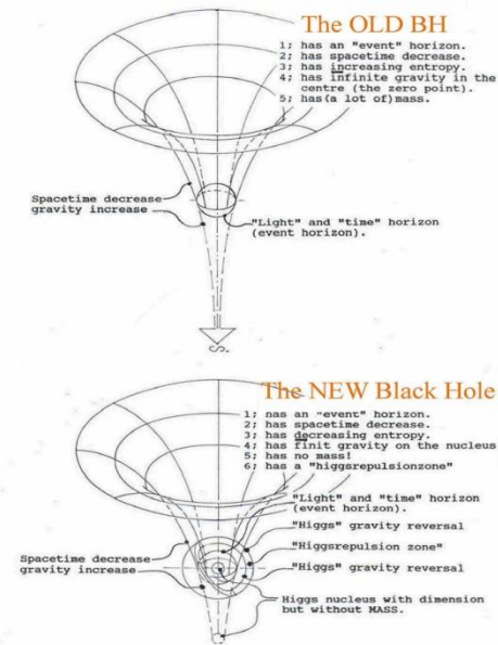
Figure 30, The new black hole
