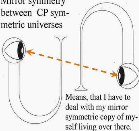
Figure 2, wavefunction collapse between CP symmetric mirror particles by instant entanglement between multi universal bubbles located around the Big Bang central void.
