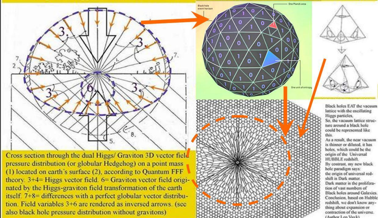
Figure 28, Quantum dimonopole repeller gravity ( the oscillating Casimir vacuum ) combined with less pressure from pushing gravitons.
