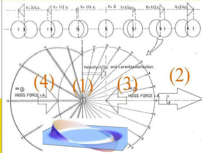
Figure 24, Quantum Gravity and Mass in motion. ( Quantum FFF Theory)
