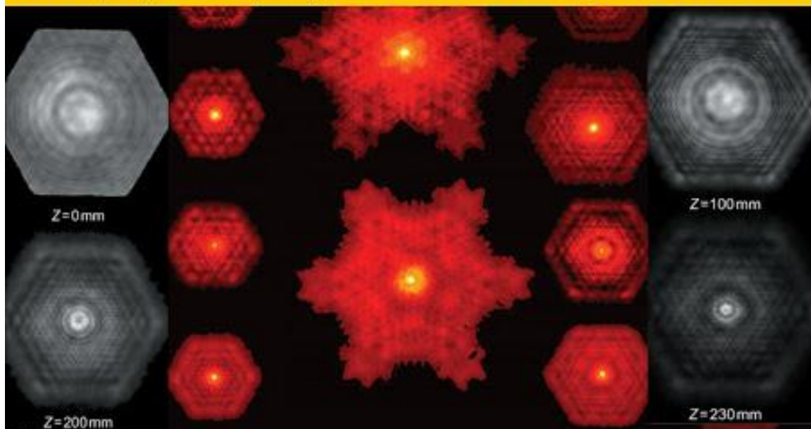
Figure 33, The Axion Higgs Pyrochlore Tetrahedral vacuum lattice seems a logical origin of hexagonal laser effect.
