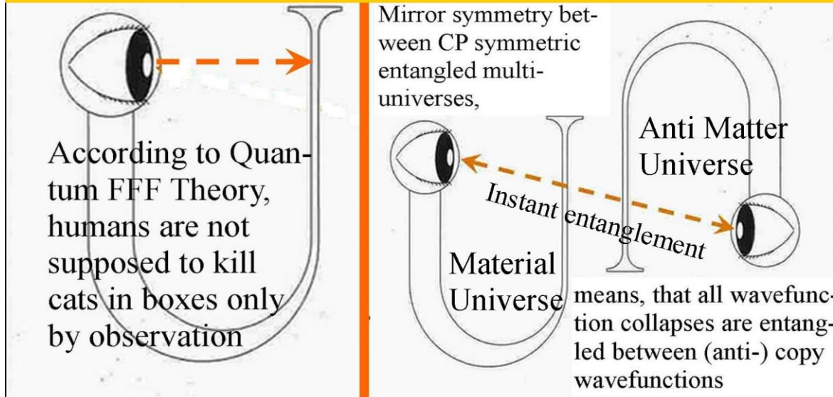
Figure, 31. Entanglement between many symmetric universes, needed for the guidance memory of all particles.
