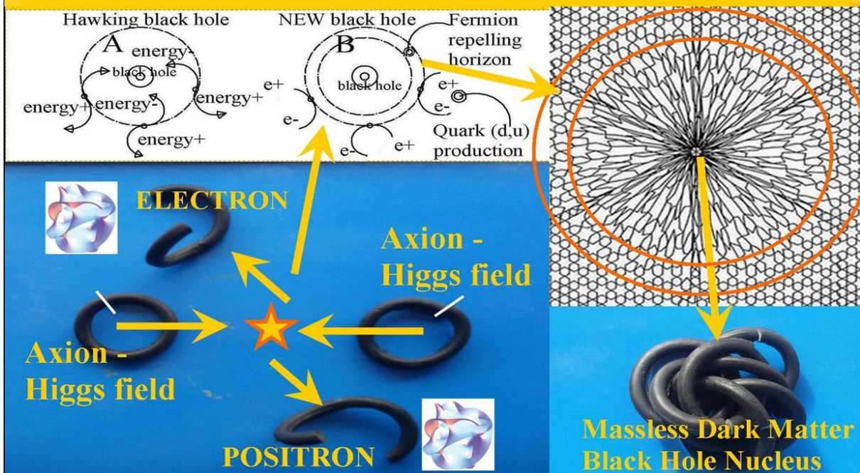
Figure 7, Fermionic propeller shaped Quantum Knots (high up right) and Higgs Boson family based Quantum Knot-Black Hole (high up, left) and pair production around black holes.
