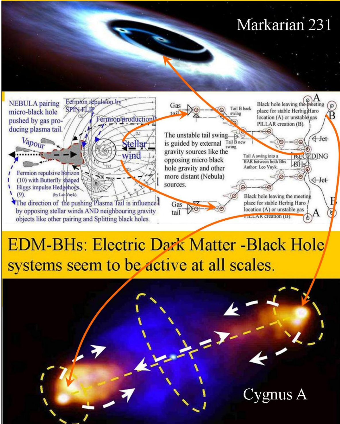
Figure 13. . the relation between Markarian 231 and other BH splitting systems
