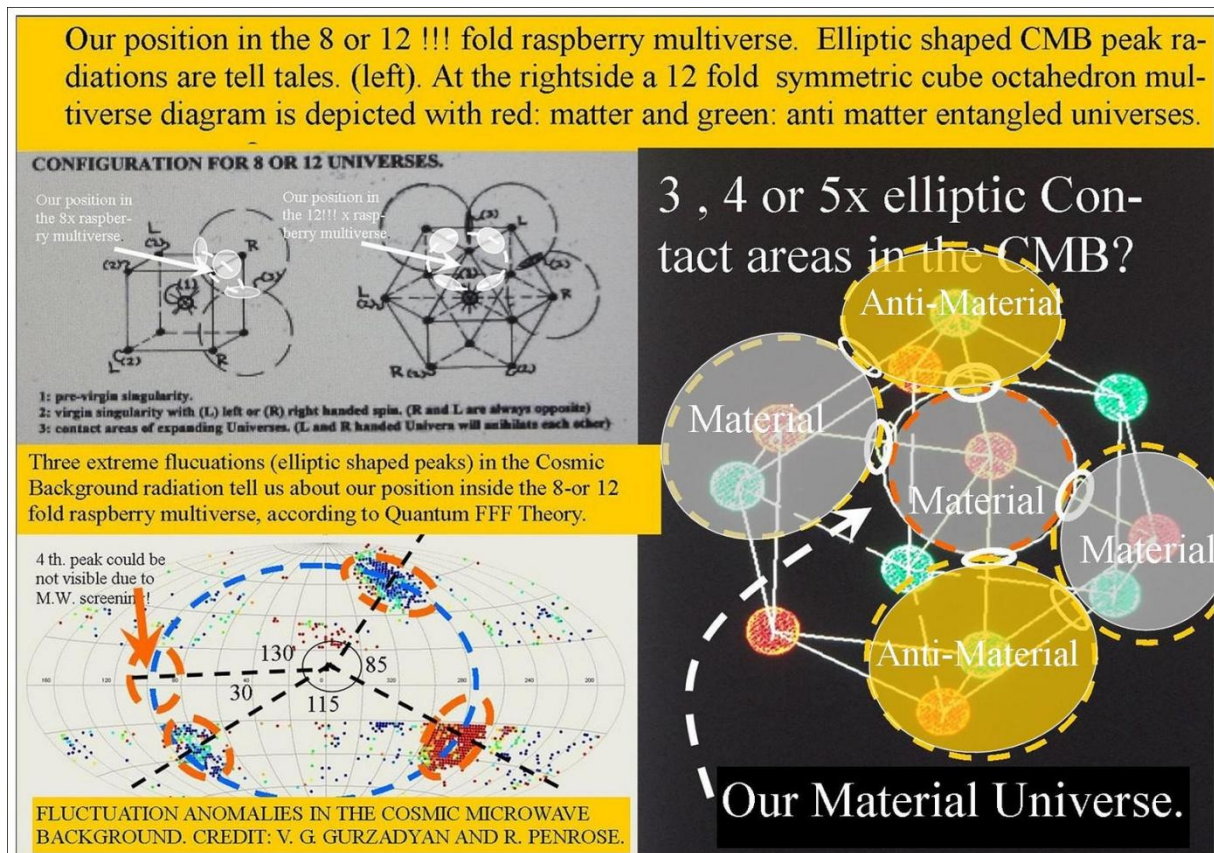
Figure 17, The Multiverse with 8-12 Charge Parity (time) symmetric Universal bubbles.
