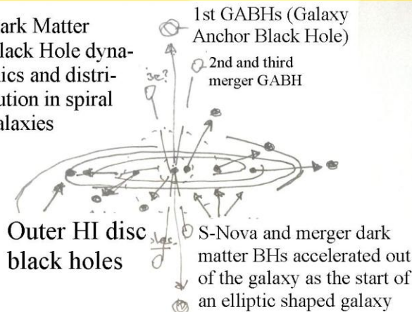
Figure, 29 . Dark Matter Black Hole dynamics in spiral galaxies.
