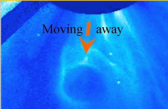
Figure 23, Even the sun seems to have polar dual black hole Herbig Haro remnants and is able to produce and expel gas planets (failed stars) at this age.
