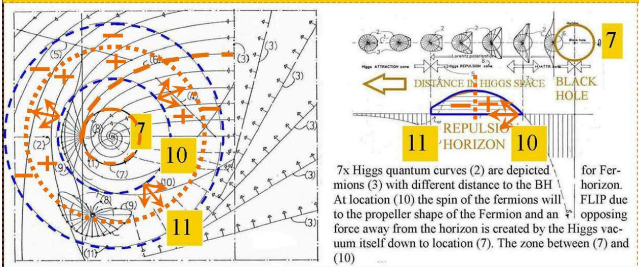
Figure 8, Electric Dark Matter Black Holes (EDMBHs) have a Fermion repelling horizon and are negative charged in our part of the multiverse.
