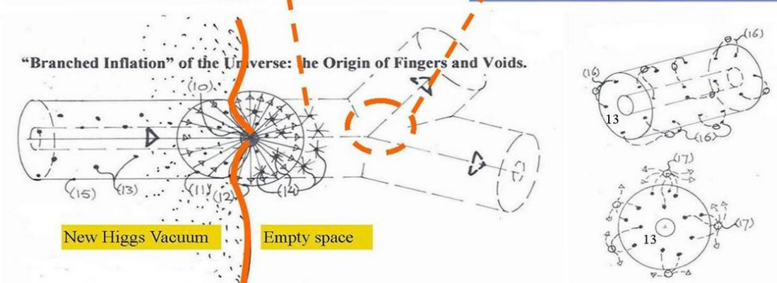
Figure 16, BBBH , the Big Bang Black Hole splintering into smaller BHs and evaporating into the oscillating Axion Higgs Vacuum lattice .
