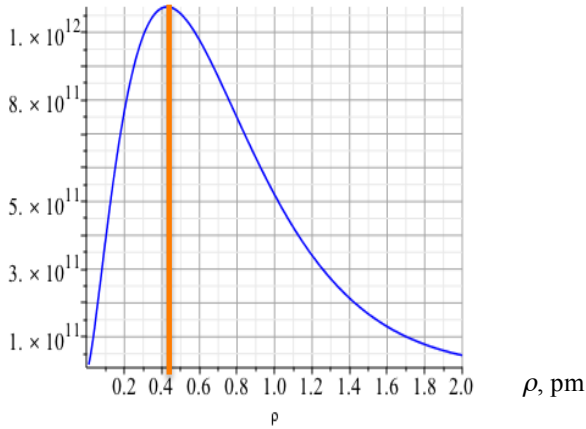
Fig. 7. Plot of norm. radial prob. density for 1s orbital of uranium, for rho < 2 pm. The maximum corresponds to rho ~ 0.43 pm
