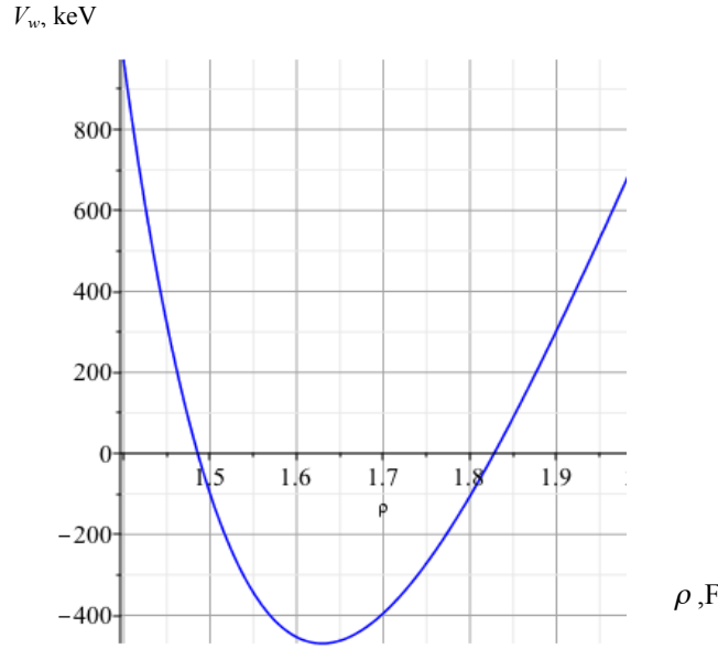
Fig. 5. Plot of electron BE, for 1.4 F < \rho < 2 F
