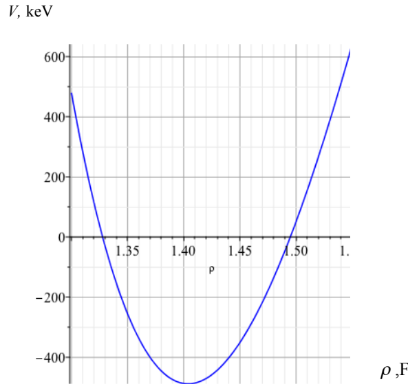
Fig. 6. Plot of electron BE, for 1.3 F < \rho < 1.55 F
