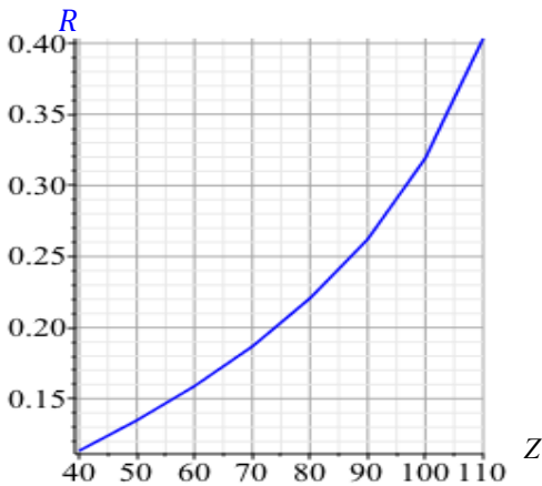
Fig. 8. Smooth plot of ratio R = |VP|/SE , as function of Z , dor 40 \leq Z \leq 110
