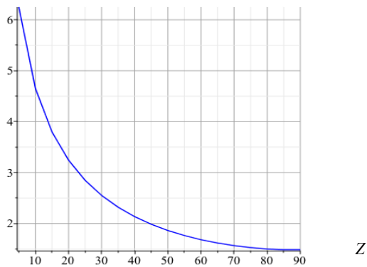
Fig. 9. Smooth plot of F'(Z) as function of Z , for 5 \leq Z \leq 90
