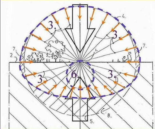
Cross section through the dual Higgs/ Graviton 3D vector field pressure distribution (or globular Hedgehog) on a point mass (1) located on earth's surface (2), according to Quantum FFF theory. 3+4= Higgs vector field. 6= Graviton vector field originated by the Higgs-graviton field transformation of the earth itself. 7+8= differences with a perfect globular vector distribution. Field variables 3+6 are rendered as inversed arrows. (see also black hole pressure distribution without gravitons)
