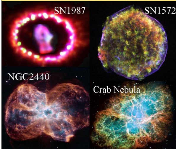
Figure 9, Other examples of Quantum Gravity effects on ejected rings of micro black hole starspots at work in different nebula .
