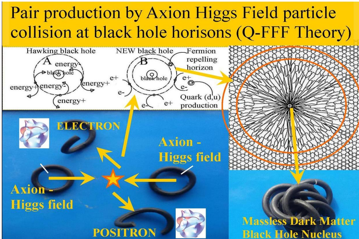
Figure 2, pair production around black holes.
