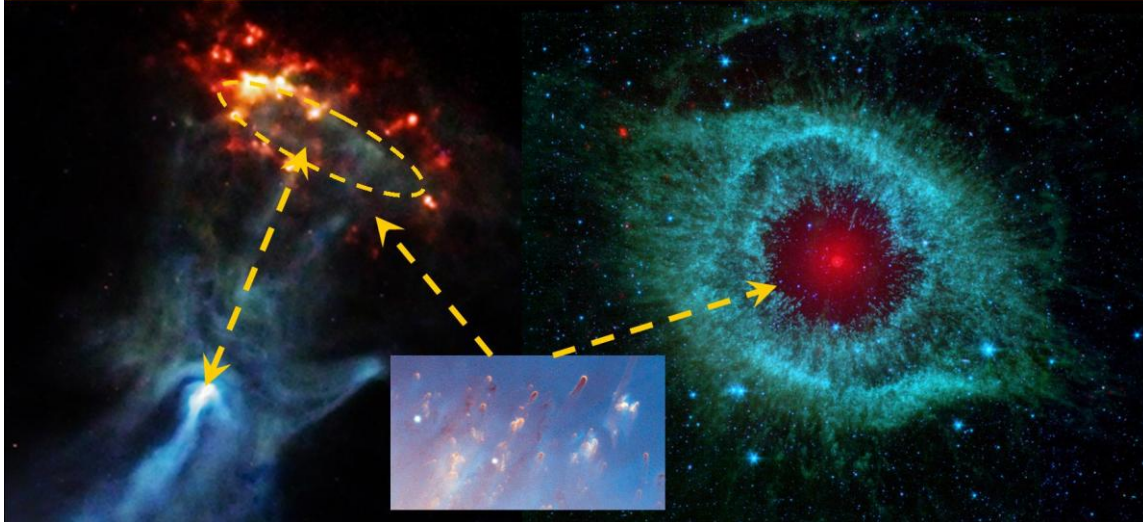
Figure 8, The A-symmetric B 1509-58 nebula , and symmetric Helix nebula as examples of the difference between Fermion- and non- inertial dark matter black hole Quantum Gravity effects.
