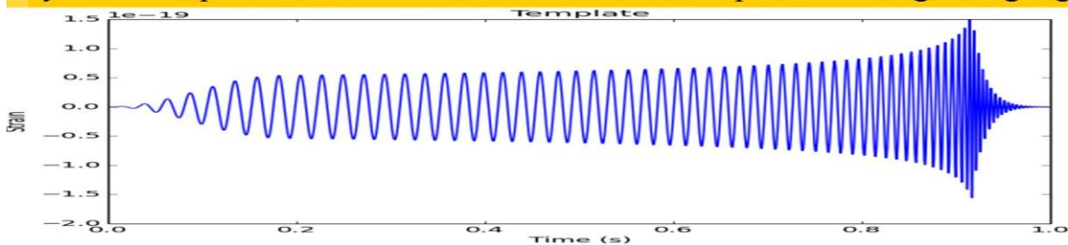
Figure 6, Massless Black Holes without Inertia effect have no rotational strain but only oscillation strains
