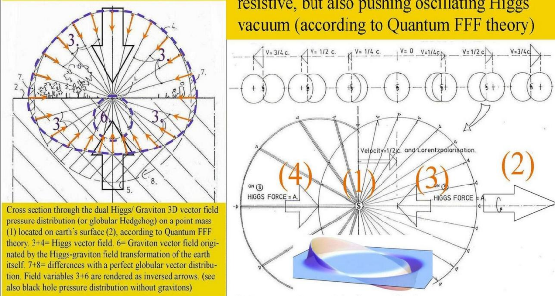
Figure 15, Quantum Gravity and Mass in motion. ( Quantum FFF Theory)
