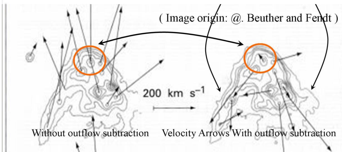
Figure 1. Latest find: evidence for new physics black hole based bowshock. Original bowshock Image presented by Beuther and Fendt ( uni of Heidelberg.)
