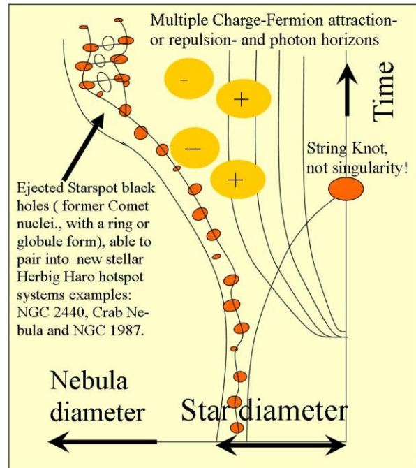
Figure 9, Other examples of Quantum Gravity effects on ejected rings of micro black hole starspots at work in different nebula .
