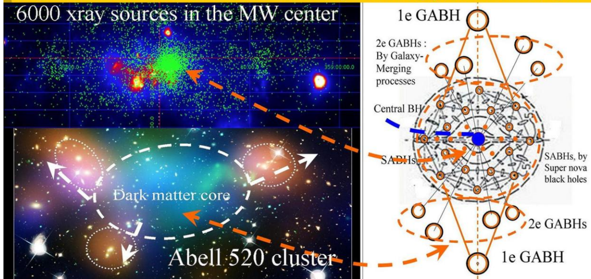
Figure 5, Merger dynamics of NON inertial Dark Matter Black Holes left behind after merging in the middle.
