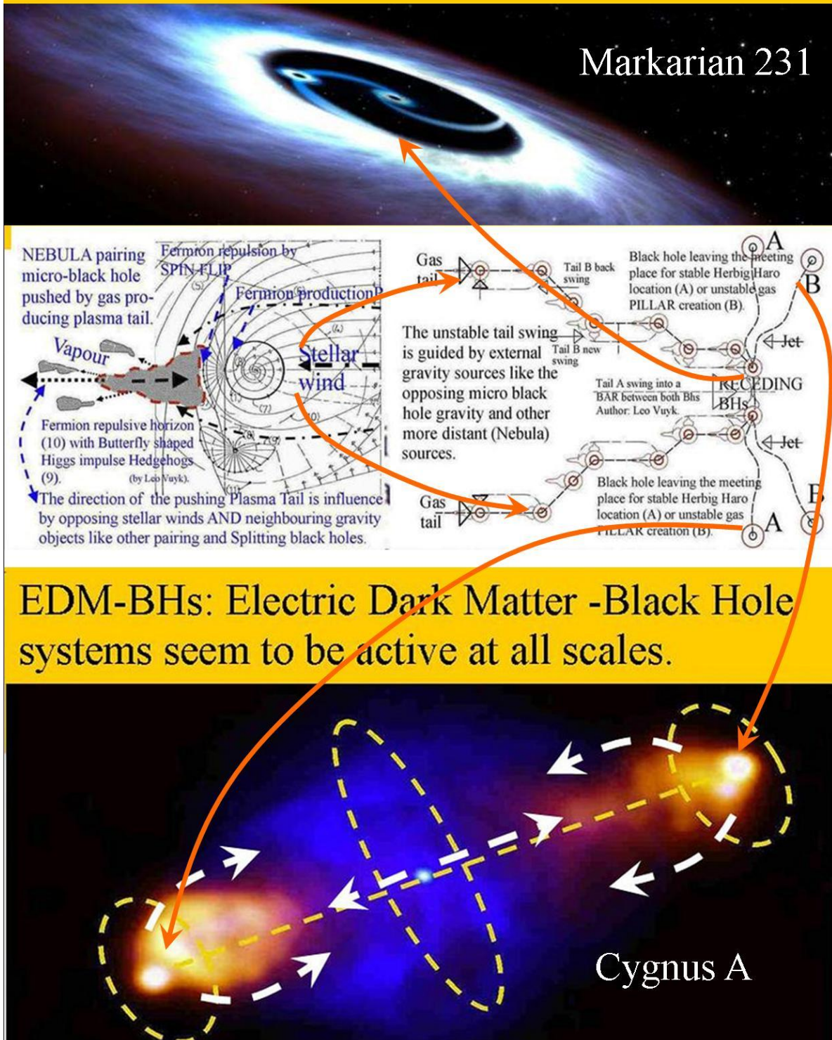
Figure 11. . the relation between Markarian 231 and other BH splitting systems
