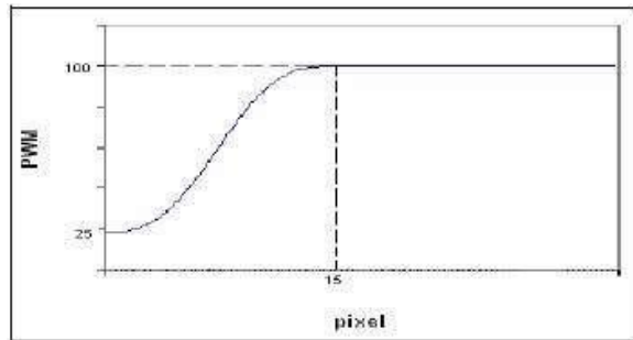
Fig. 7 Speed control of tilt motor
