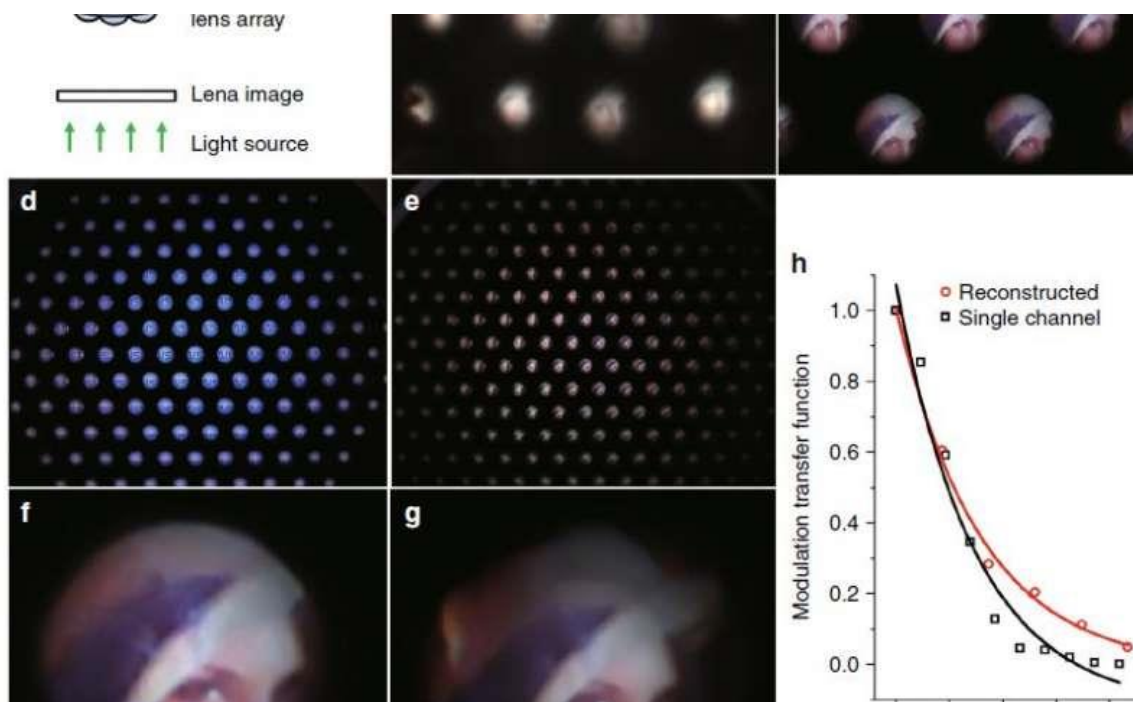
Figure 2. Optical images captured by the bioinspired ultrathin digital camera. Credit: Light: Science
