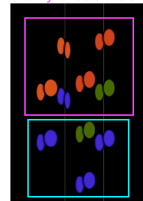
8 Standard Model Root Vectors
