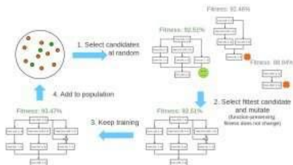
Figure 2: The NCEvolve workflow. Credit: IBM Bleeding-edge research technology
