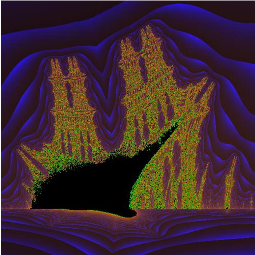
Figure 1. BurningShip - Fractal
