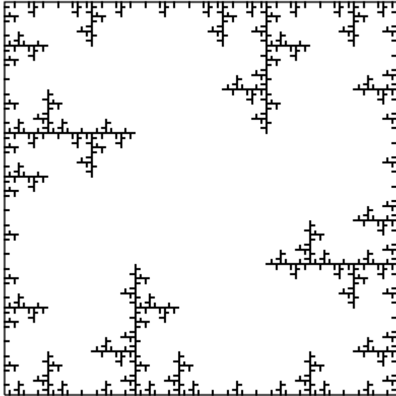
Figure 3. Fractal - Crystal
