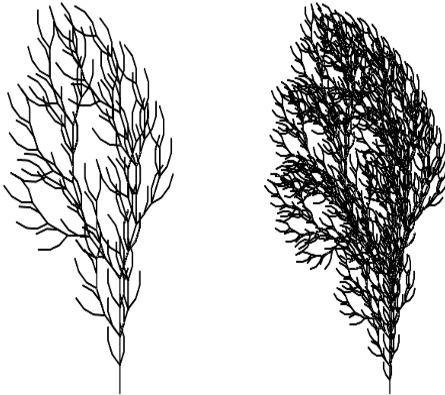
Figure 3. Fractal - Seaweed
