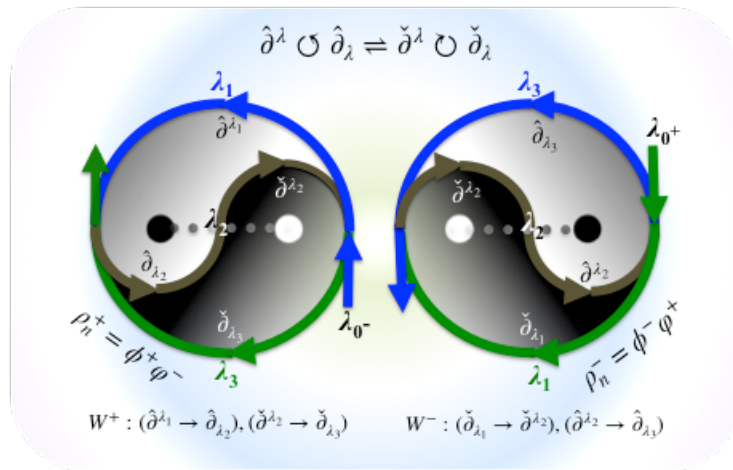
Figure 2.0a: YinYang Event Processes \hat{\partial}^\lambda \circ \hat{\partial}_\lambda = \check{\partial}^\lambda \circ \check{\partial}_\lambda
