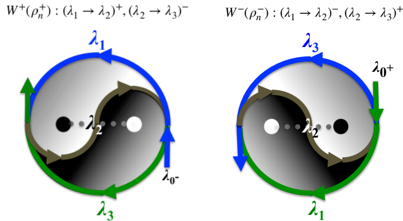
Figure 1.7: Events of YinYang Processes ( Quadrant-States )
