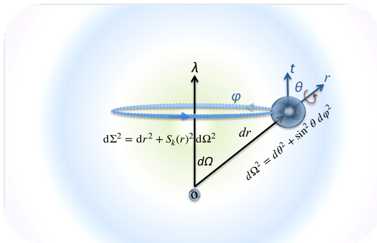
Figure 1.12: Evolution from World Planes into Spacetime Manifold
