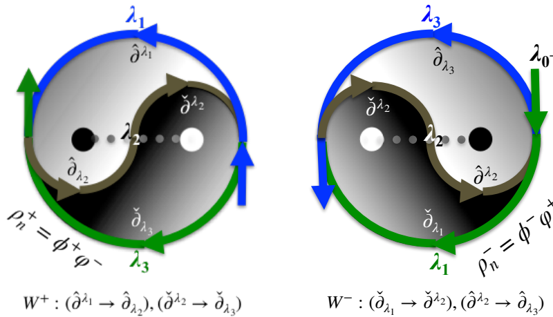
Figure 2.0a: Events of YinYang Processes : \hat{\partial}^\lambda \cup \hat{\partial}_\lambda = \check{\partial}^\lambda \cap \check{\partial}_\lambda
