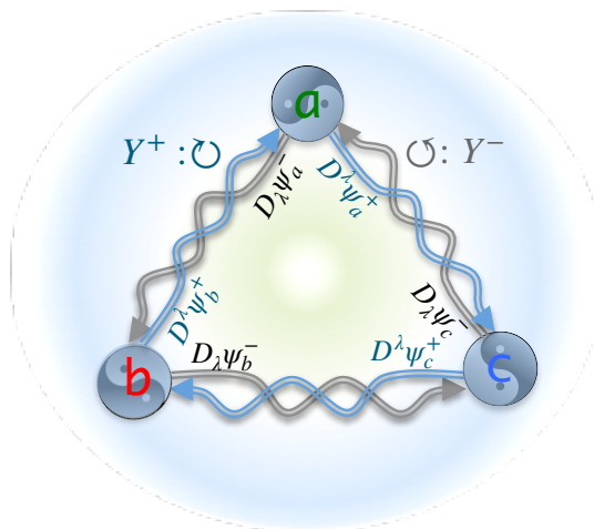
Figure 2.0b: Ontological Evolutions \hat{\partial}_\lambda \check{\partial}^\lambda \mapsto (\dot{x}^\mu \zeta^\mu D^\lambda \hat{\psi}) \wedge (\dot{x}^\nu \zeta^\nu D_\lambda \check{\psi})
