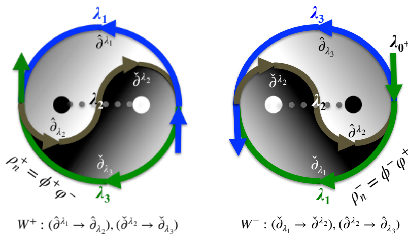
Figure 2.0a: YinYang Event Processes \hat{\partial}^\lambda \cup \hat{\partial}_\lambda = \check{\partial}^\lambda \cup \check{\partial}_\lambda
