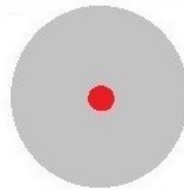
Quantum
