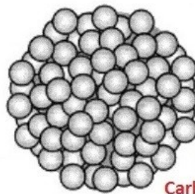
Quantum
