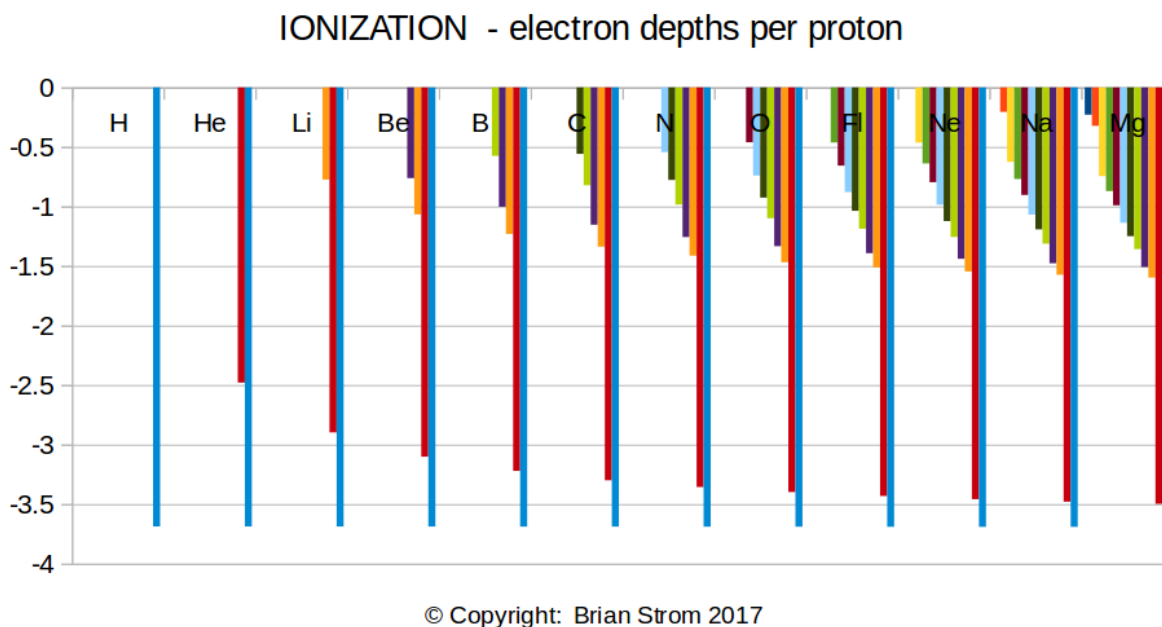
Figure 4b. IONIZATION: Histogram of electron depths per proton.
