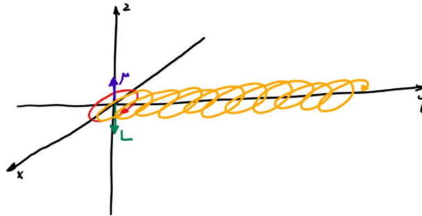
Figure 5: Is this the Zitterbewegung in a Stern-Gerlach apparatus?
