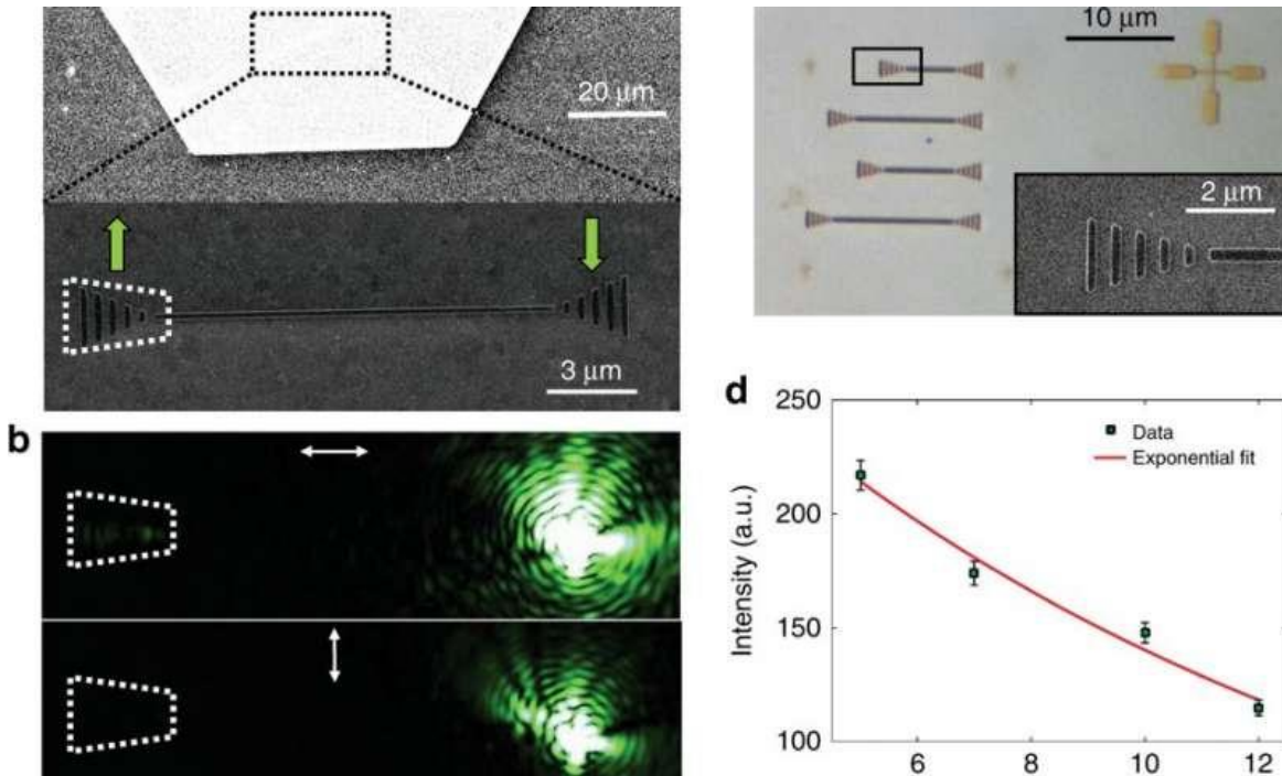
Transmission of green laser light (532 nm) along the low-loss plasmonic waveguide, a) SEM image of a single crystalline flake (top) and fabricated DLSPW waveguide atop of the Ag plate (bottom), b) optical characterization of the waveguide ... more
