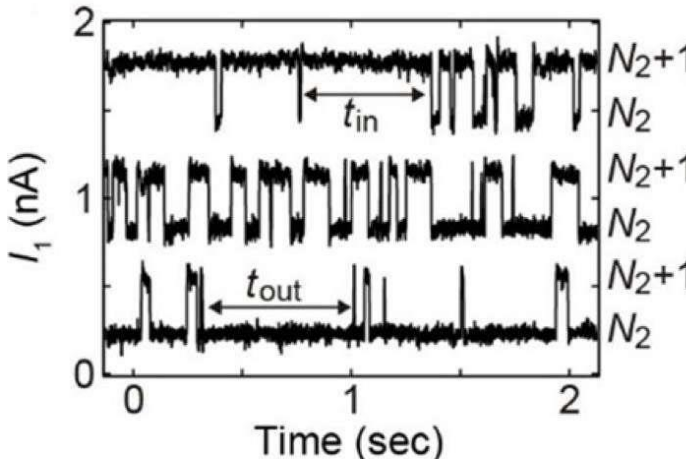
Real-time traces of the charge sensor quantum dot (QD1) current. Changes in the charge sensor current indicate the increase and decrease of electron number in the adjacent quantum dot (QD2). Credit: Osaka University
