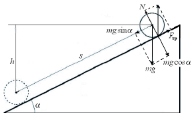
Fig. 1. Galileo's experiment. The motion of the ball on an inclined plane.
