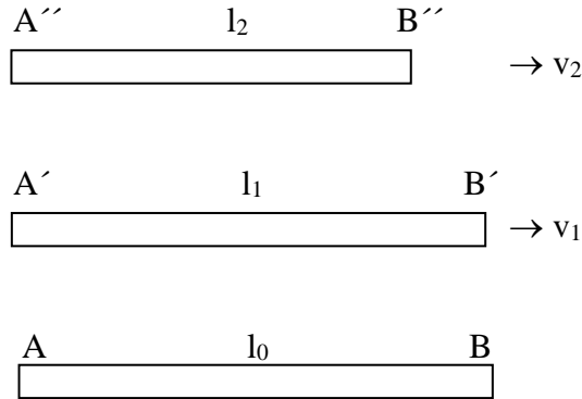
Figure 3. S'' with the proper length l_2 ( \alpha = 0 ) that “synchronize” a Lorentzian clock located at B' marking zero when B'' pass by B'
