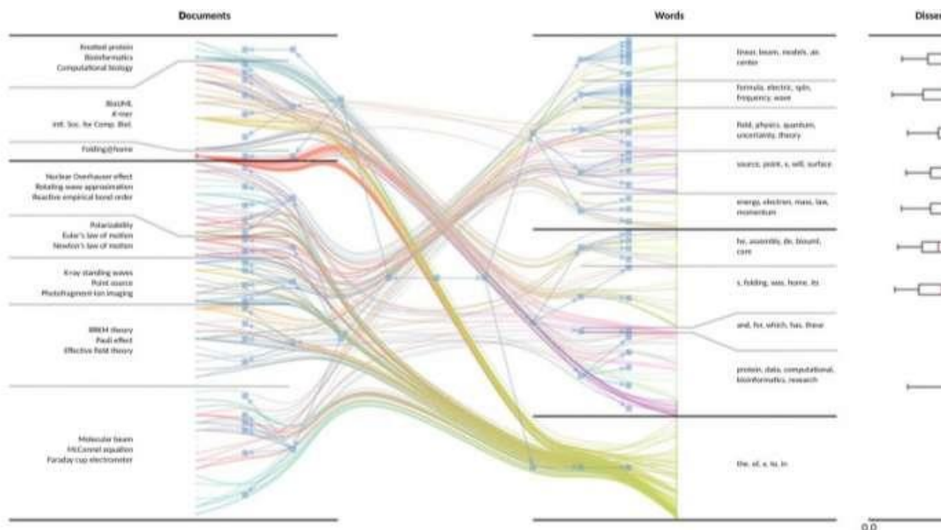
Fig. 5. Inference of hSBM to articles from the Wikipedia. Articles from three categories (chemical physics, experimental physics, and computational biology) are analyzed. The hierarchical level reflects bipartite nature of the network with document nodes (left) and word nodes (right). The grouping on the second hierarchical level is in accordance with the three categories. We show examples for nodes that belong to each group on the third hierarchical level (indicated by dotted lines): For word nodes, we show the five most frequent words; for document nodes, we show three (or fewer) randomly selected articles. For each word, we calculate the dissemination coefficient U_D , which quantifies how the word is distributed among documents ( U_D = 1 indicates the expected dissemination from a random null model; the smaller U_D ( 0 < U_D < 1 ), the more unevenly the word is distributed). We show the 5th, 25th, 50th, 75th, and 95th percentile for each group of word nodes on the third level of the hierarchy. Intl. Soc. for Comp. Biol., Intl. Soc. for Comp. Biol., Intl. Soc. for Comp. Biol., Intl. Soc. for Comp. Biol., Intl. Soc. for Comp. Biol.
