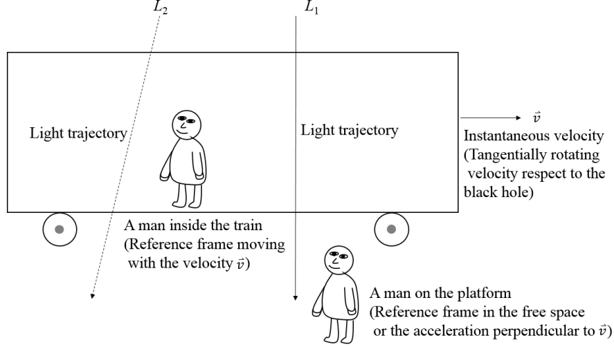
Figure 1. The observations of the light trajectory from different reference frames. A reference frame, the transparent train, has the velocity v the same as the tangentially rotating velocity of the Kerr-Newman black hole. An observer stays on the train and the other one is at rest on the platform. This observer on the platform is the reference frame in the free space or the acceleration perpendicular to v . A light beam observed by the observer on the platform is perpendicular to the movement of the train denoted as the light trajectory L_1 where no dragging-frame effect exists. The same light beam observed by the observer moving with the train is the light trajectory L_2 where the dragging-frame effect exists.
