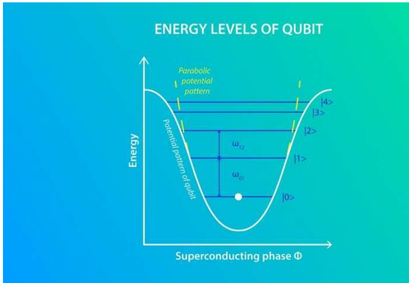
Figure 2. The energy spectrum of a transmon is similar to that of an atom. The frequency of the transition between the first two energy levels is \omega_{01} . Credit: Elena Khavina/MIPT
