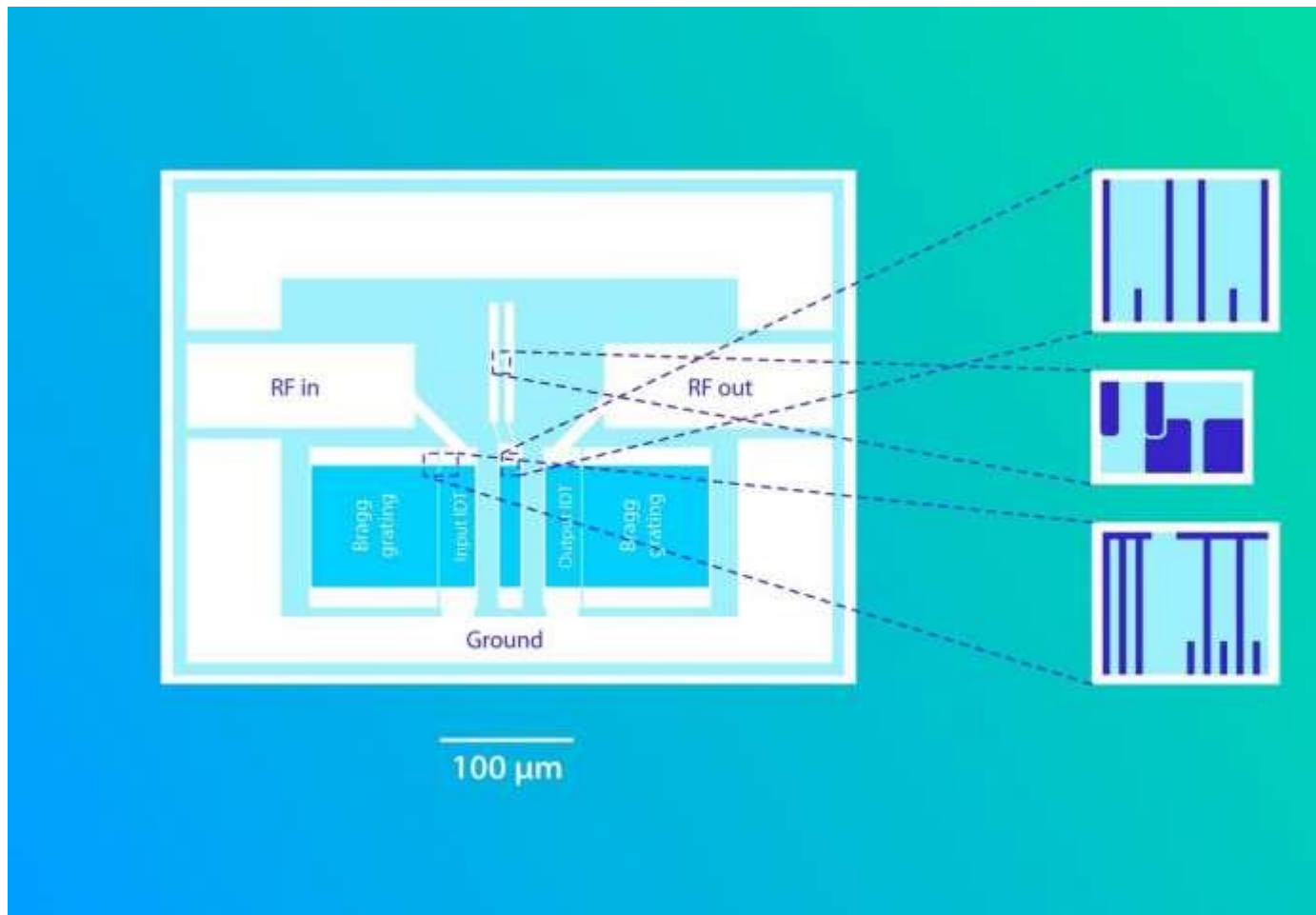
Figure 4. Acoustic chip. The size of the entire system is comparable to that of the magnified square region in figure 3. A nanometer ( 1\ \text{nm} ) is one-billionth of a meter and one-thousandth of a micrometer ( 1\ \mu\text{m} ). RF stands for radio frequency. Credit: Elena Khavina/MIPT
