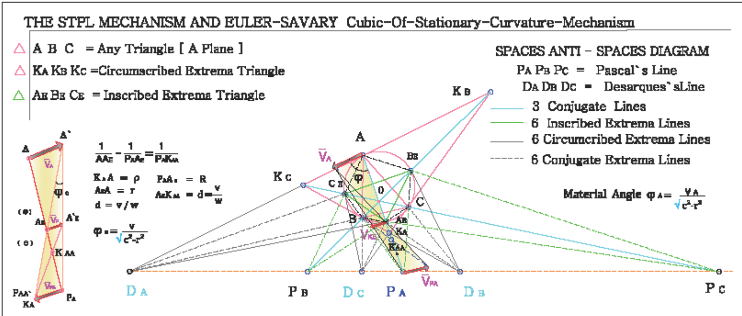
Figure.7.. ABC is any triangle ( The Space ), K_A K_B K_C triangle is the ( The Sub-Space ), A_E B_E C_E triangle is (The Anti-space) respectively . The Instantaneous Pole P \equiv A_E of rotation is off the circle on AA_E axis .Inscribed to ABC circle is Common circle of STPL- \{D_A-P_A\} mechanism The Reference System \{D_A- P_A\} \equiv [R] (x',y',z', t') moves with velocity, \bar{v} , parallel to, x-x' , axis with respect to the fixed and Absolute System \{D_A- O\} \equiv [S](x,y,z, t) . The Space point, A, moving on (p) curve, and Anti-Space point A_E moving on ( \epsilon ) curve are rolling on the same Sub-space circle (O,OA) \equiv (O,OA_E) which is the common cave-circles of Material Geometry in STPL - \{D_A-P_A\} mechanism .
