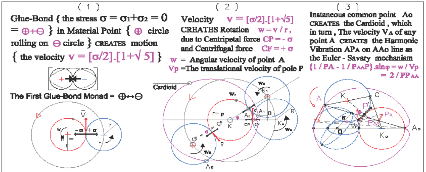
Figure.14. Pole of rotation P, on STPL line AP_A , is the Instantaneous centre of rotation for [\oplus] , Space on [\ominus] Anti-space, through Sub-space, \emptyset , and or, every couple of lines between Spaces and Anti-spaces. Cardioid is the envelope of circles (K_0, R) , (K, r = R) whose centres K_0, K lie on a given circle (P, PA_0) which pass through a fixed point, A_0 , on the given circle (P, PA_0) . Nutation happens at N, common point. Analytically in [58].
