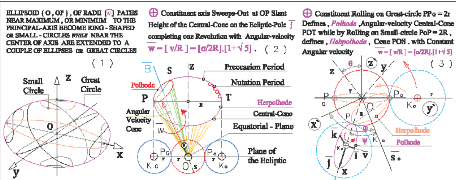
Figure.20. In (1), are shown different Paths near maximum or minimum Principal axis from where become-ring shaped or Small-circles while near the center of axis extend to a couple of ellipses or Great-circles. For a constant Angular-velocity, w , and by changing torsional momentum, B , only then Infinite curves are possible for the motion.
