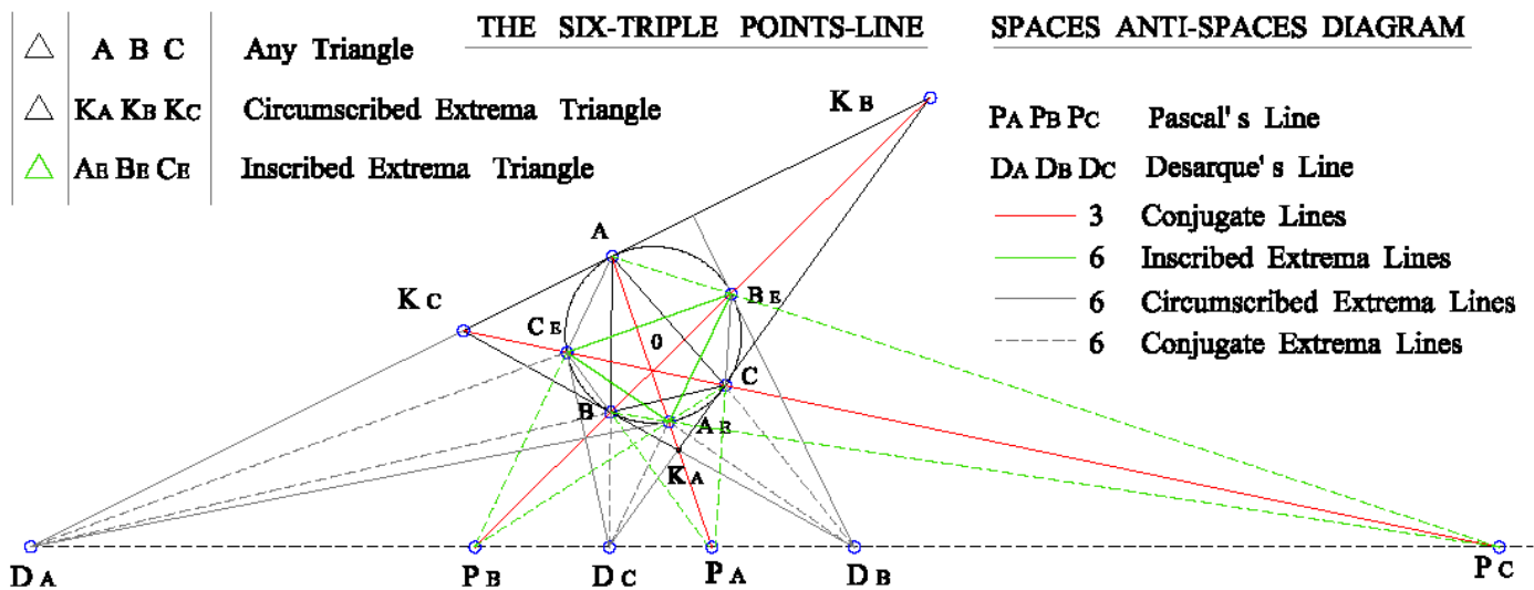
Figure.6.. The Six, Triple Concurrency Points, Line . [STPL] \rightarrow D_A, D_B, D_C - P_A, P_B, P_C [ ABC \equiv The Space ], [ A_E, B_E, C_E \equiv The Anti-Space ], [ K_A, K_B, K_C \equiv The Sub-Space ]
