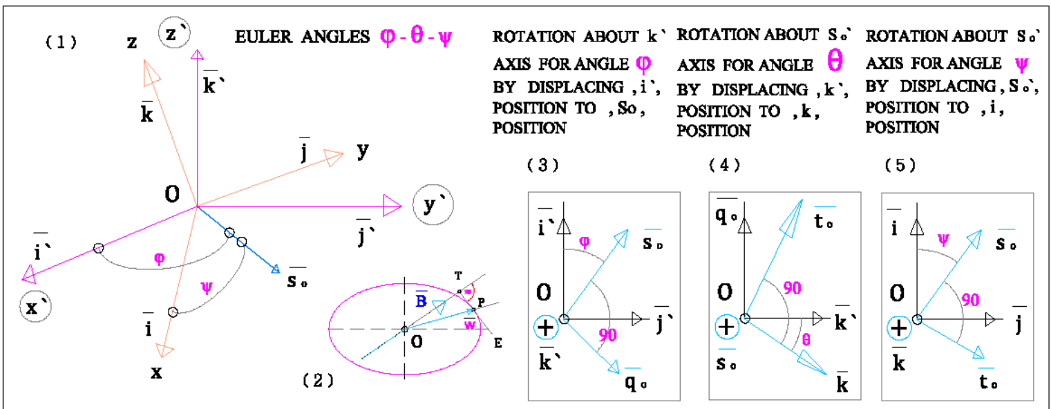
Figure.17. . In (1) are shown Euler angles { \varphi, \vartheta, \psi } in a Fix-Three-Coordinate-System x, y, z through ,O, and one Movable x', y', z' at , O .
