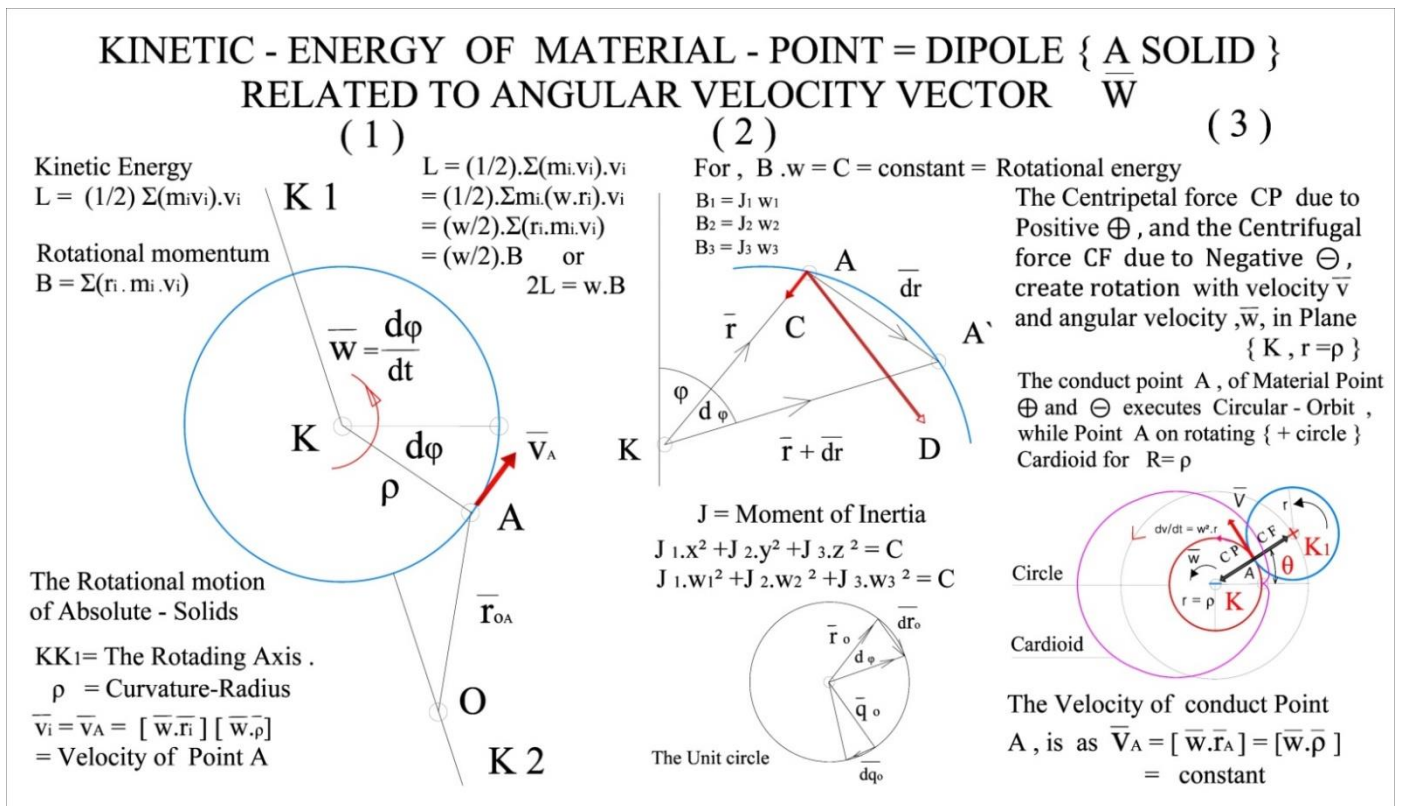
Figure.13.. The Cycloidal motion in, Material Point \equiv The monad is Dipole \equiv [\oplus \ominus] = \emptyset = K_r AK_{R=r} where \rightarrow K_R \equiv [\oplus] \leftrightarrow K_r \equiv [\ominus] \rightarrow \equiv 0 . The total torque becomes from \pm Spin which equilibrium in System of circle K_r , Evolute circle K_R , as Cardioid of the same center. In (3) the Flexible - String OA is stretched under equilibrium Tension = \pm \sigma and rotated around O center with a constant angular velocity, w , and is vibrated in Normal modes.
