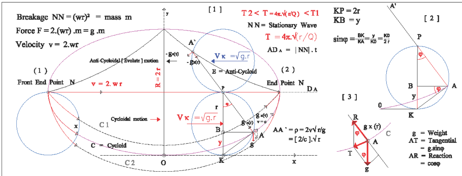
Figure.11.. The Cycloidal motion in , Material Point ≡ The monad is Dipole ≡ [\oplus \ominus] = \emptyset = AA' where → A \equiv [\oplus] \rightarrow A' \equiv [\ominus] \rightarrow |AA'| \equiv \emptyset \equiv The Brachistochrone Curve C \equiv N1 \rightarrow N2 . Motion on Curve C1 acquires a period T1 > 4\pi\sqrt{r/g} , while on C2 T2 < 4\pi\sqrt{r/g} which is not Isochronous .
