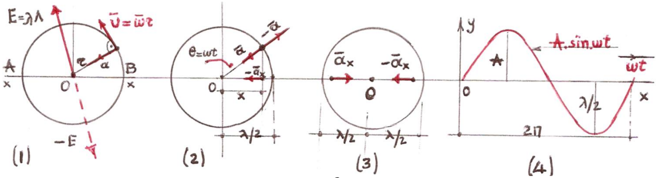
Figure.23. In (1) , are shown Velocity , |\vec{v}| = w.2r = \frac{2\pi}{T}.r = 4\pi r. f = [\frac{\sigma}{2}].(1+\sqrt{5}) , Angular velocity |\vec{\omega}| = \frac{\sigma}{2r} [ 1 + \sqrt{5} ] and Frequency , f = \frac{(1+\sqrt{5}).\sigma}{4\pi r} in cave , r .
