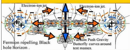
Cygnus A with dual plasma/gas producing "New physics" negative charged BHs as hotspots, with growing merger (SN) black hole in the center. Below: local Quantum vacuum push gravity vector butterflies originated by the BH vacuum absorption of dark vacuum energy.
