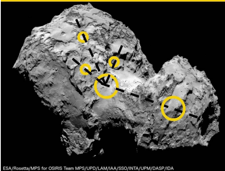
Figure: 17, Proposal for the origin of circular craters at Comet 67p C-G.
