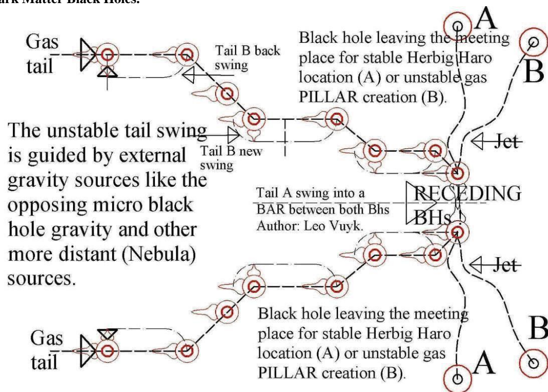
Figure 7, New Black hole propulsion principle by a self produced plasma-dust tail,. As a consequence, New black holes do not merge to form larger nuclei, they even repel negative charged metal surfaces by their own exterior electron charge. ( see also fig. 9)
