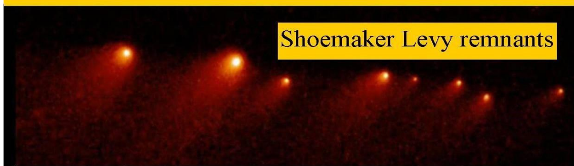
Figure 20, Hyperion a single nuclear comet, in contrast with Shoemaker Levi multiple nuclear comet.
