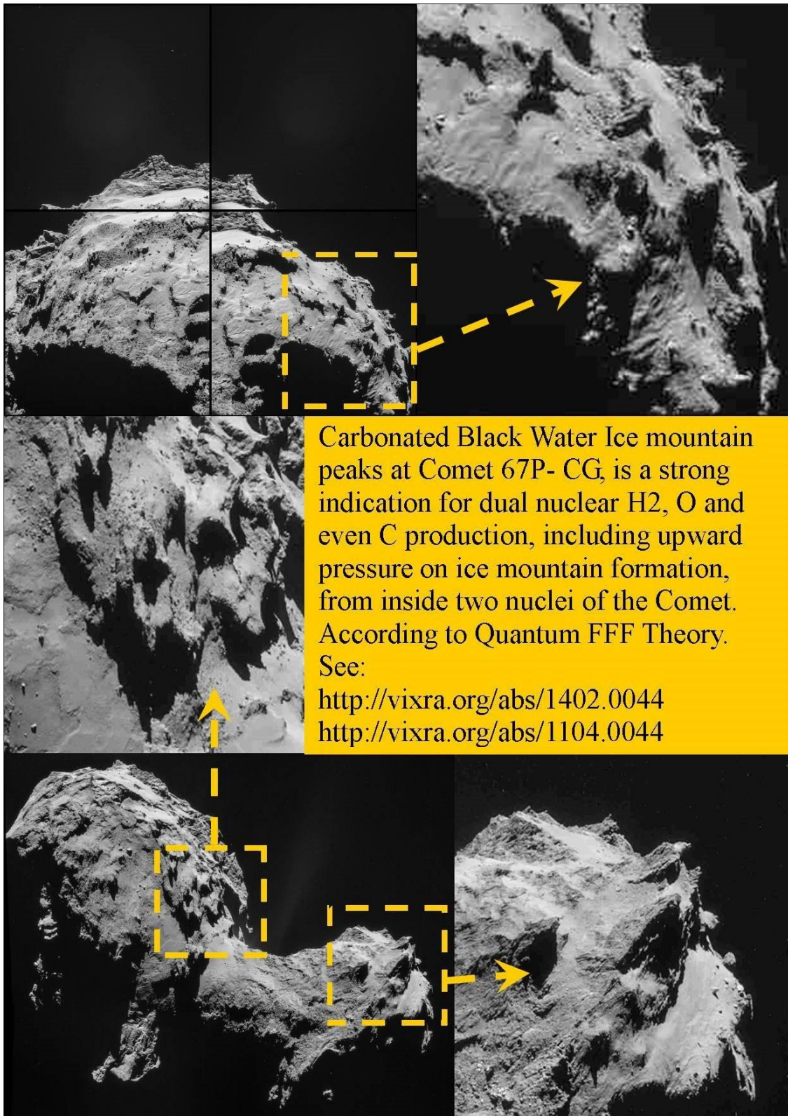
Figure 21, NOT EROSION but Plate tectonics driven by the nuclear matter production of new paradigm dark matter black holes.
