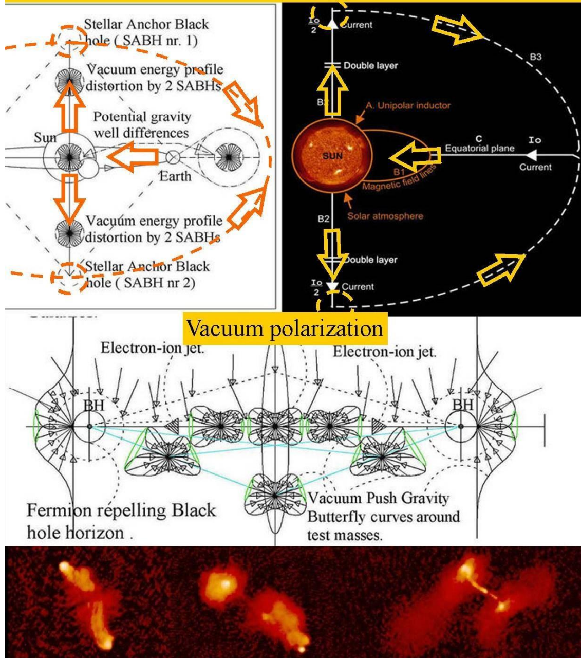
Figure: 9. Black hole propulsion and pairing principle of fig 8, seems to be the origin of dual Stellar or galaxy Anchor black holes (see figure 11) and even so called Birkeland /Alfvén current circuits around stars and galaxies by vacuum polarization. The energetic polarized vacuum oscillation spectrum is the motor for fast gas and electron transport starting direct after the big bang.
