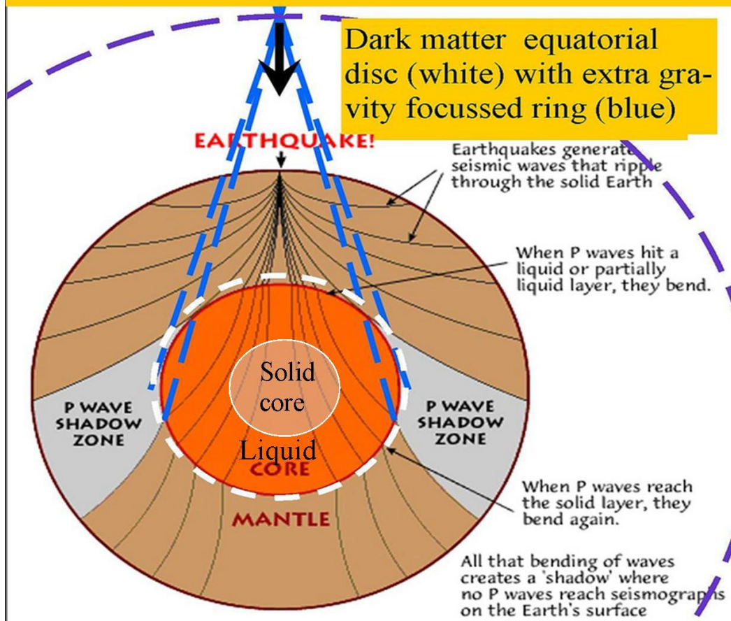
Figure 4, According to Quantum FFF Theory, Electric dark matter black holes, even in the form of microscopic size and produced by magnetic quantum interference, they produce plasma and water and are proliferated through stellar systems, as unstable Ball Lightning up to stable Comets and Sunspots (crashed Comets) As a consequence, crashed comets in the earth are responsible for the volcanism and so called growing Earth by its growing compressed water core.
