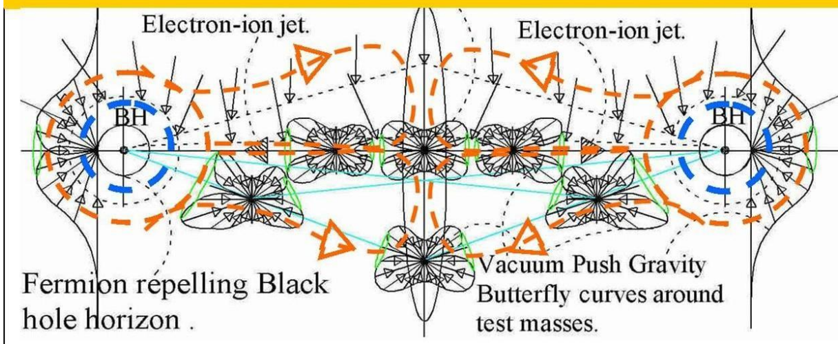
Figure: 15, Comet 67P C-G, with electrical model of the dual dark matter black hole system with O H Hydroxyl and water ice production.
