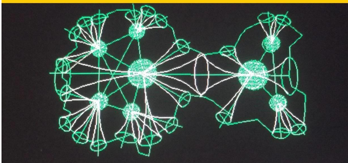
Figure 27, Internal Porous Funnel Structures, created by Dark Matter BH point sources for Comet 67PCG, and Hyperion. (A former Comet left alone by its former Dark Matter BH nucleus).
