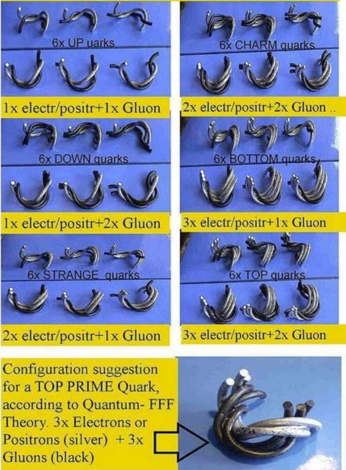
Figure 12, 5x different shaped Photon/Gluons can combine with the two propeller shapes of the Electron and Positron to form all coloured (QCD) Quarks and even a so called Top Prime Quark. The Muon and Tau particle are supposed to be the same as the Down quark, respectively the Charm quark.
