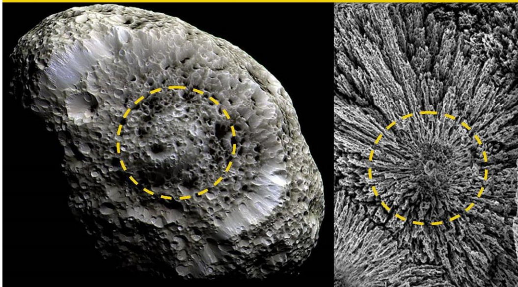
Figure 19, Hyperion, a former Comet.
