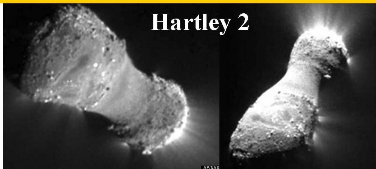
Figure: 14, both comets more in detail.
