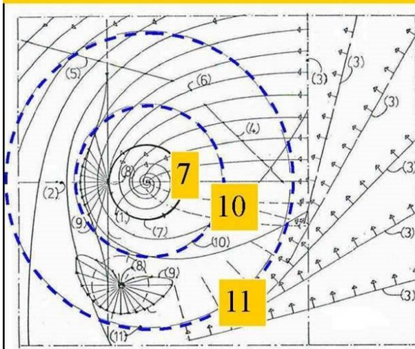
Figure: 16. Fermion repulsion principle around dark matter black holes producing water ice Comets Megacryometeors. A special example of nuclear water ice production is found in the Moon Hyperion, which is assumed to be a former Comet, left alone by its Black Hole energy source.
