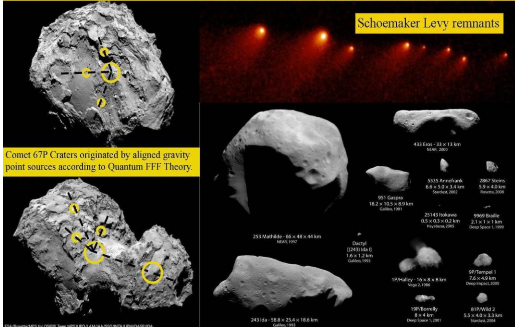
Figure 18, What can we learn about multiple nuclear comets?
