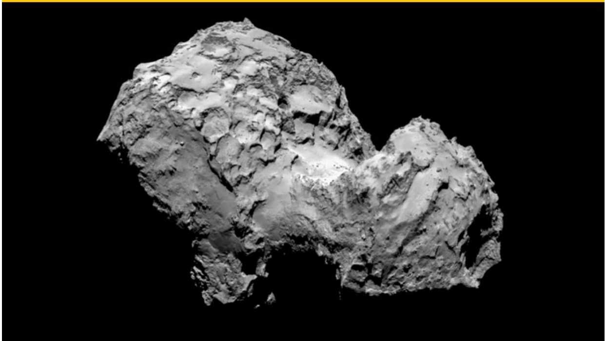
Figure 13: Dumbbell shaped Comets, 25 Hartley and Comet 67P C-G.
