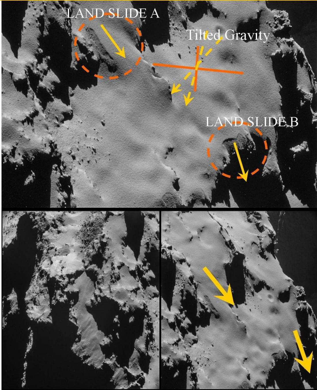
Figure 25, Anomalous non perpendicular surface Gravity problem.
