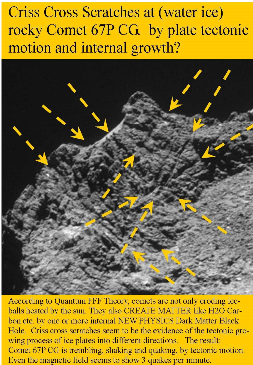
Figure 24, Criss cross scratches at comet 67P CG, as evidence for internal ice growing and plate tectonic motion into different directions.
