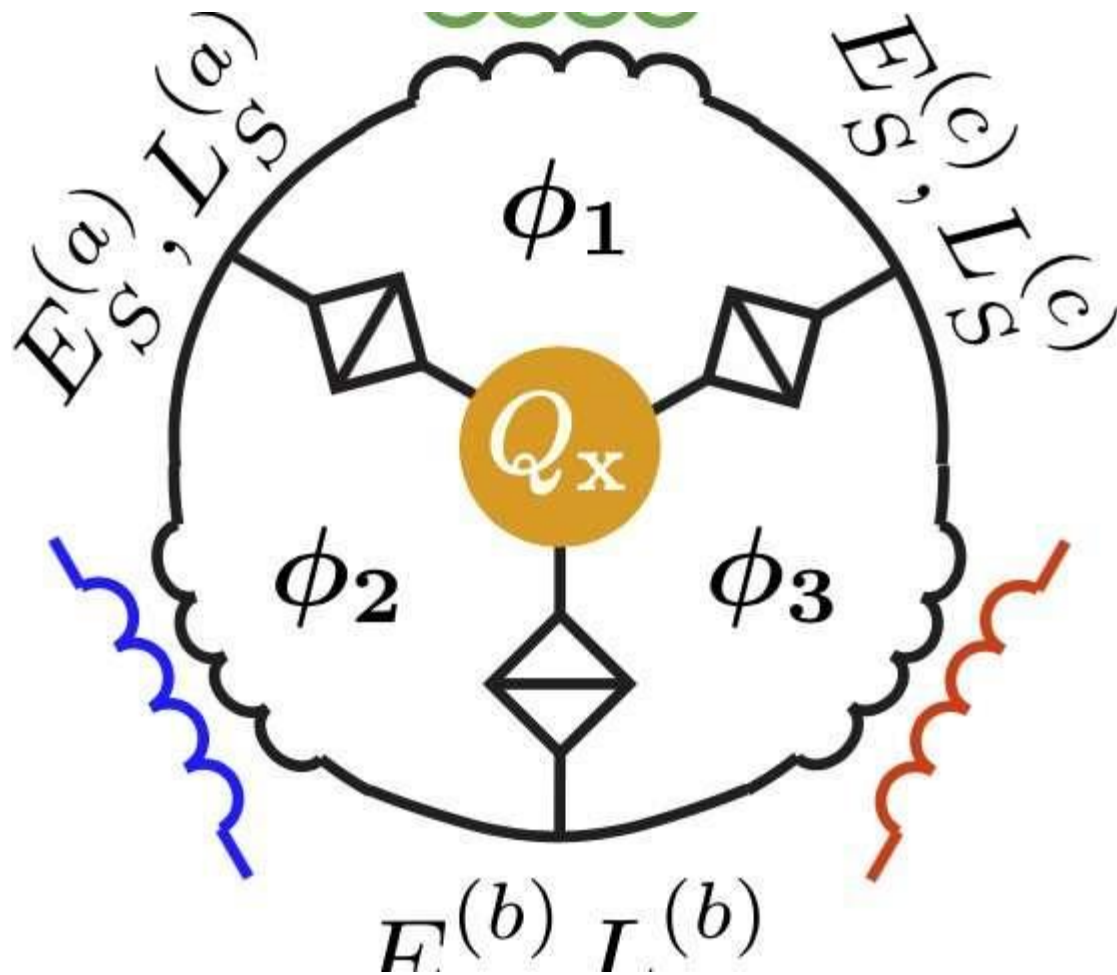
Schematic representation of the proposed circulator. Credit: FLEET
