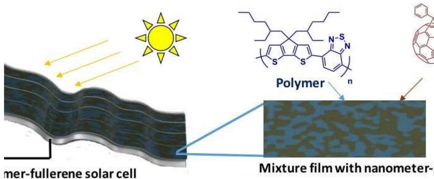
Fig. 2. Photoelectric conversion in polymer solar cell and chemical structures of the active materials. Credit: Osaka University
