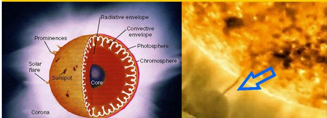
Figure: 19, ( see also ref. [13]) Bright points or spots at the solar surface represent small Comets able to leave the sun by new pushing Cometary tails like Ball Lightnings do. The origin of these bright points are supposed to be so called “Interference black holes” according to Q-FFF theory.
