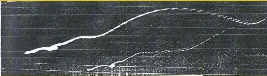
Birth of EM interference based Ball Lightning or micro Black Hole. (Photo: W.H. van Overhagen 11 aug 1991 during thunderstorm from roof window, the Netherlands)
