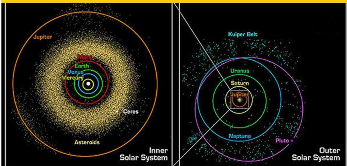
Figure: 20, The solar baby comets are supposed to travel onto the different clouds or belts like the Oort cloud and Kuiper- and Inner Jupiter belt.
