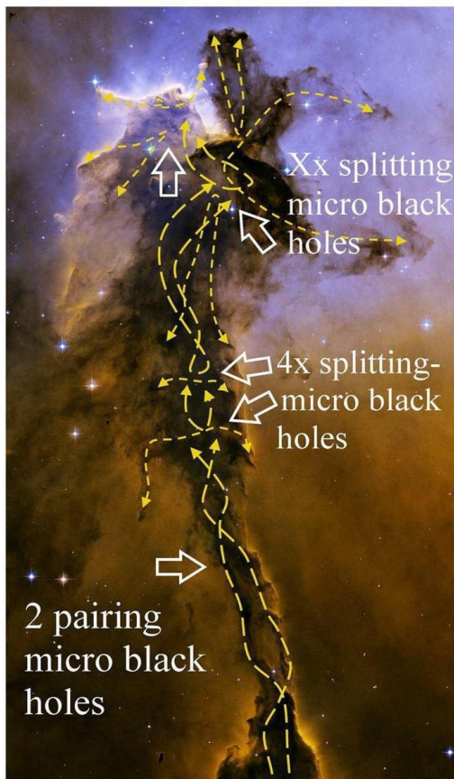
Figure 12, Comparison with splitting and pairing Micro black holes inside Planetary nebula, and the formation of comet nuclei like the Hyperion icy nucleus.
