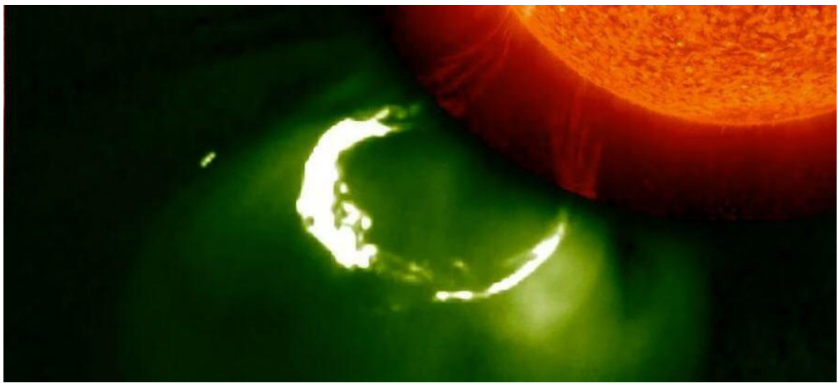
Figure: 18, Fireball production of the sun, leading to micro Comets comparable to Sprite fireballs on earth
