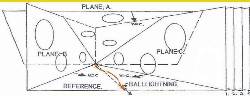
Birth of EM interference based Ball Lightning or micro Black Hole. (Photo: W.H. van Overhagen 11 aug 1991 during thunderstorm from roof window, the Netherlands)
