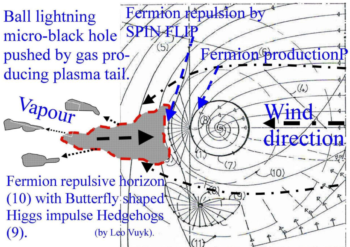
Figure 8, It is assumed that the New Paradigm Black hole is able to use and accumulate so called “Zero Point Energy” to form Plasma tails which seem to be able to push the black hole away from the centre of mass of the earth. (Ref. 4 )
