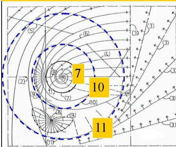
Figure: 22, Electric Skyrmion Black Hole based Ball Lightning
