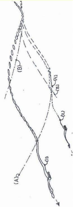
Birth of EM interference based Ball Lightning or micro Black Hole. (Photo: W.H. van Overhagen 11 aug 1991 during thunderstorm from roof window, the Netherlands)
