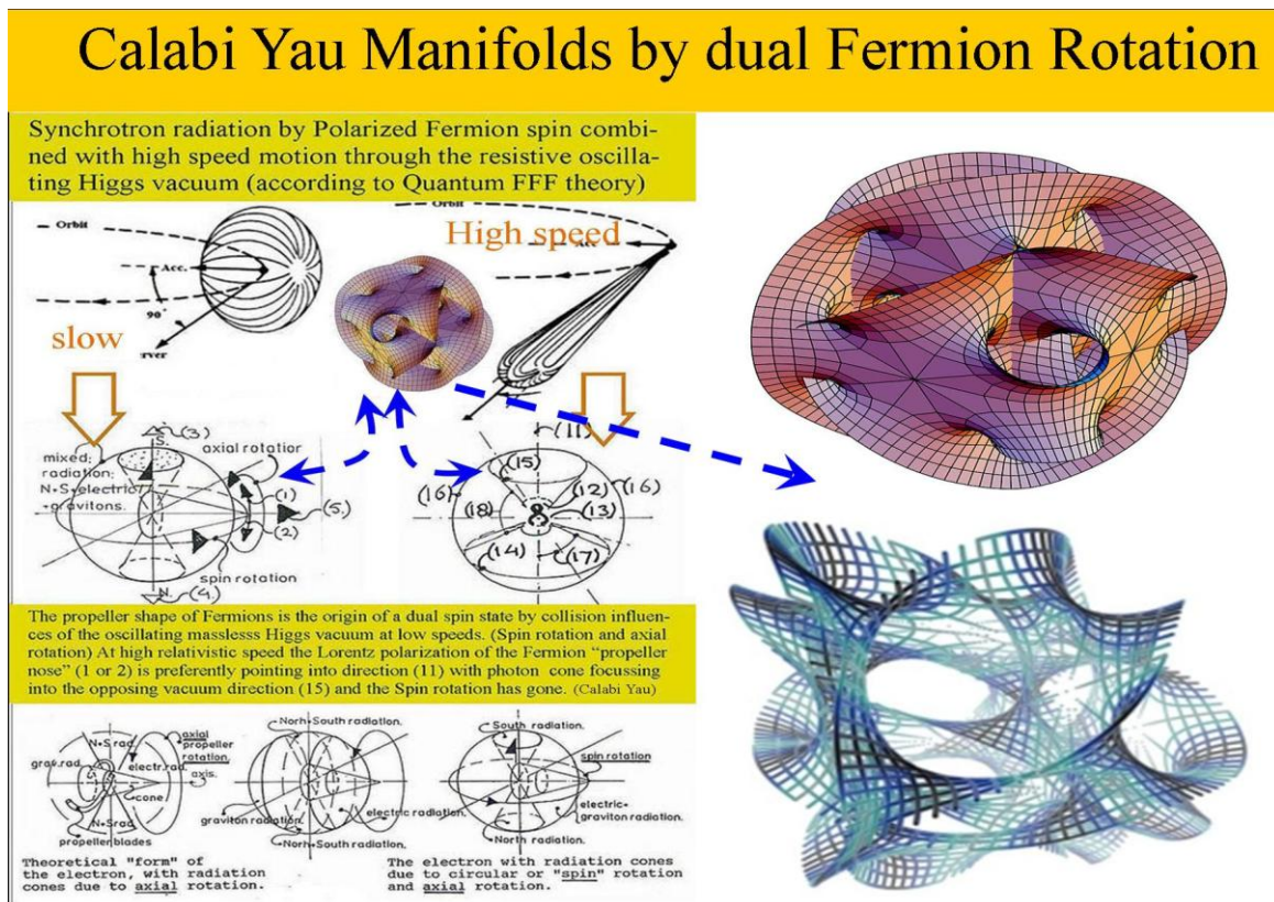
Figure 27. Calabi Yau Manifolds.
