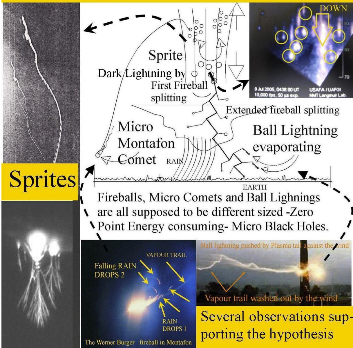
Figure: 15, Several examples of Quantum Knot Ball Lightning created by electro magnetic Interference, Micro Comets and Sprite fireballs combined with Gamma ray "Dark lightning".
