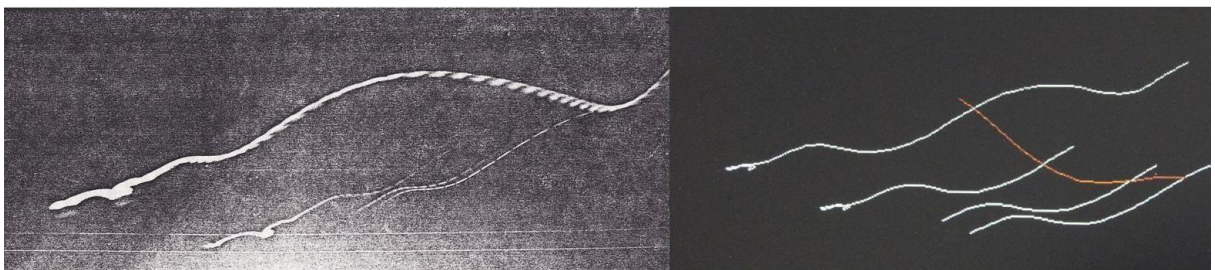
Figure 6, Example of micro black hole production possibly by strong electromagnetic or x-ray interference at sea level. There are four traces to be observed with comparable waveforms. ( see also at the right side: reconstruction image). The left photo is made by Mr. Overhagen (the Netherlands) by automatic shutter camera through his roof window, during heavy thunder storm. The two bumps at the end of two waveforms could be the start of the formation of a micro Black hole.
