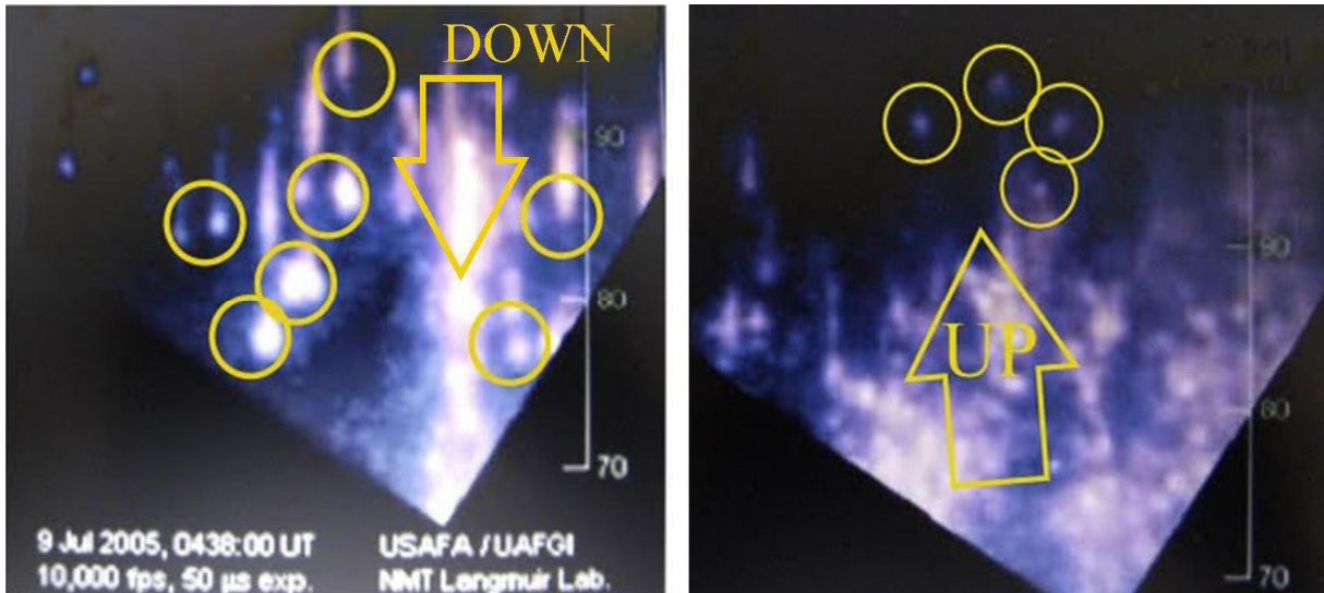
Figure 4, FIREBALL images observed inside a Sprite by a video. The video is made by a High speed camera (10.000 f/sec) of the Langmuir laboratory (USA, 2005) looking at 70-120 km altitude.
