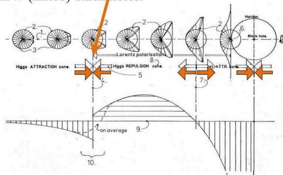
Figure 12, Comparison with splitting and pairing Micro black holes inside Planetary nebula, and the formation of comet nuclei like the Hyperion icy nucleus.
