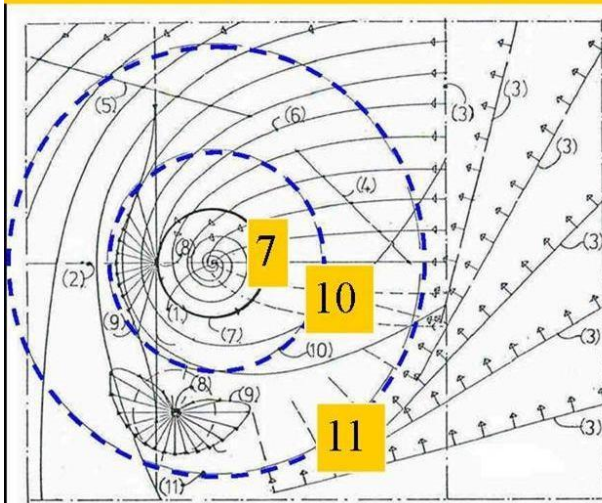
Figure: 23, Electric Black Hole based Comets and Micro comets.
