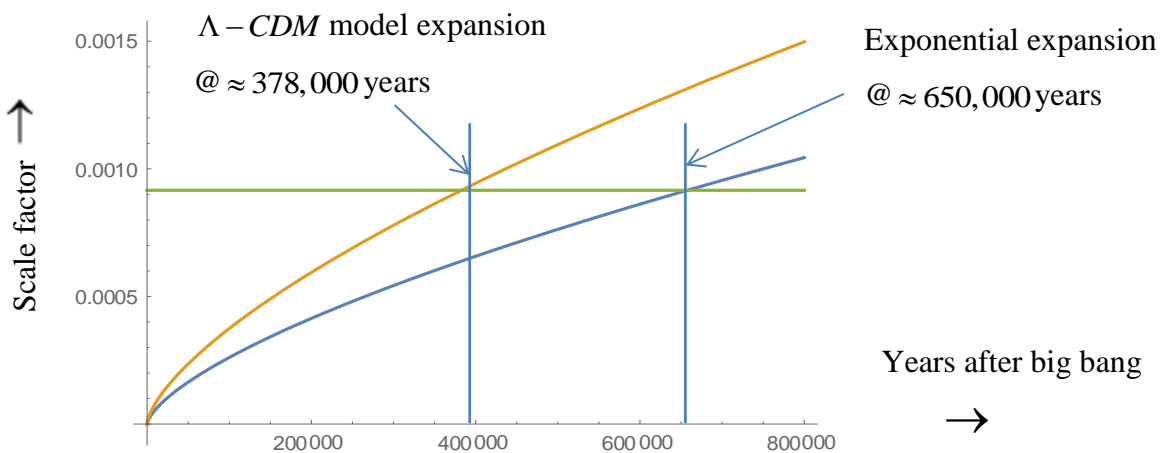
Figure 5.3. 8 Scale factors as a function of years after the big bang for the \Lambda - CDM model, and our ( b = 0.53 ) exponential expansion model. The scale factor of 1/1091 (relative to now) at recombination is identical in both cases, but occurs later with exponential expansion.
