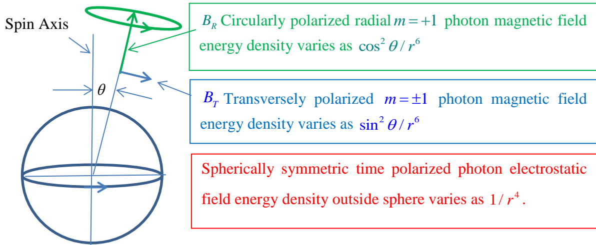
Figure 7.1. 1 Spinning electrically charged sphere. At same radius B_R @ (\theta = 0) = 2B_T @ (\theta = \pi / 2) .
