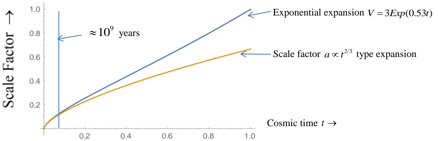
Figure 5.3. 6 Up to approximately the first billion years, the scale factor for continuous exponential expansion in the matter dominated era is almost identical to a \propto t^{2/3} .
