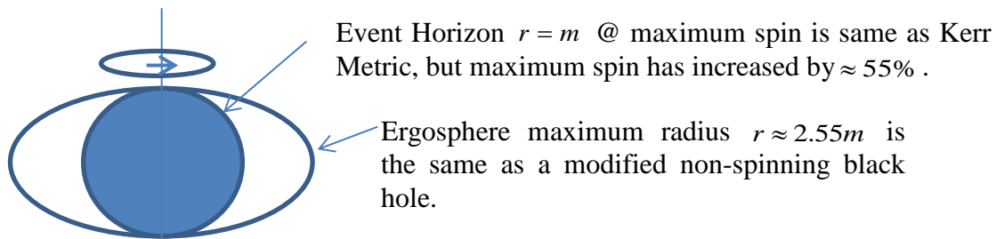
Figure 8.1. 1 Modified Kerr Metric with the dimensionless parameter A changed from A = \frac{2m}{r} \rightarrow A = \frac{2m}{r} + 1.4 \frac{m^2}{r^2} . It initially appears to clash with GR near the horizon.
