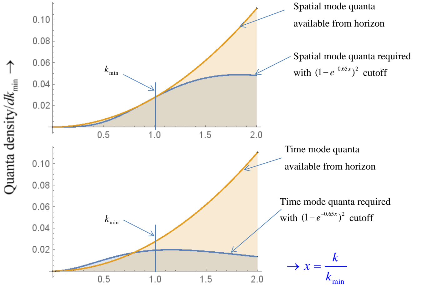
Figure 5.3. 1 plots Eq's.(5.3. 2) & (5.3. 11) as a function of x = k / k_{\min} . Going through similar procedures for the time mode quanta as for space modes, we have plotted both time and space. The exponential e^{-0.65x} cutoff fits available and required reasonably for k < k_{\min} in both cases; also showing there should be an adequate supply of time mode quanta from the horizon for all infinitesimal mass particles. The spatial mode intersects @ k = k_{\min} . Both plots always look the same at all cosmic times T . And, in any metric only the value of k_{\min} changes. It only works in an expanding flat universe. Equating required and available spatial modes @ k = k_{\min}
