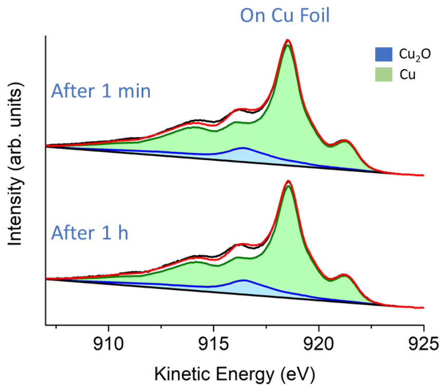
Figure S4: Cu AES LMM Spectra of 250 nm Cu-Cubes on a Cu Foil measured quasi in situ after 1 minute and 1 hour of \text{CO}_2\text{RR} at -1.0\text{V} vs RHE.
