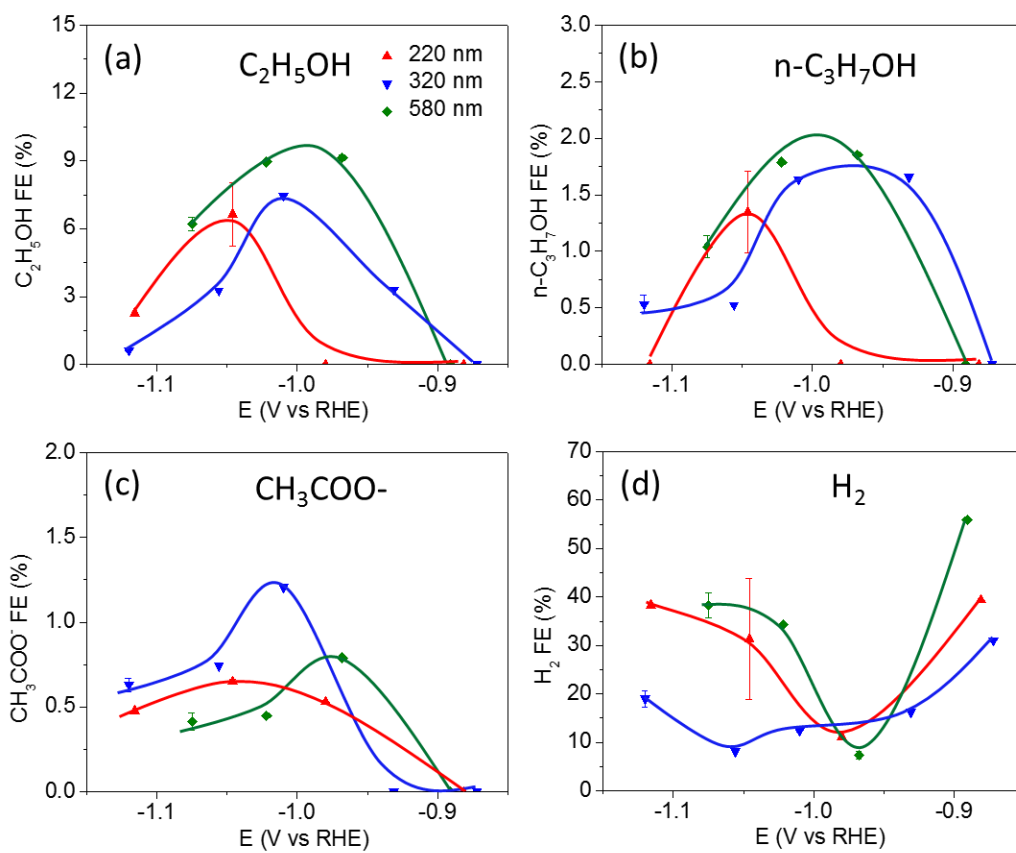
Figure S10: Faradaic efficiency for ethanol (a), 1-propanol (b), acetate (c), and hydrogen (d) after 1 hour of CO 2 RR at different potentials.
