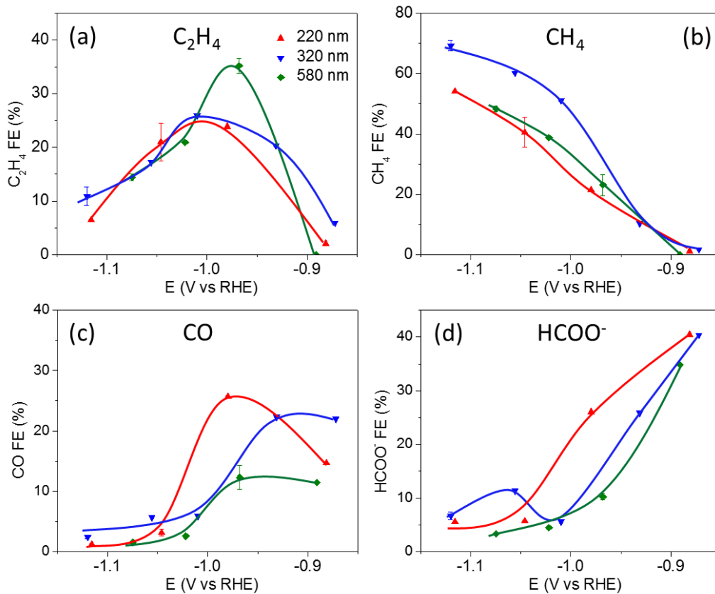
Figure S9: Faradaic efficiency for ethylene (a), methane (b), carbon-monoxide (c), and formate (d) obtained after 1 hour of CO_2RR at different potentials. The products produced by a reference blank substrate scaled to the (approximate) unoccupied carbon paper in the samples was subtracted to show only the products from the Cu-cubes.
