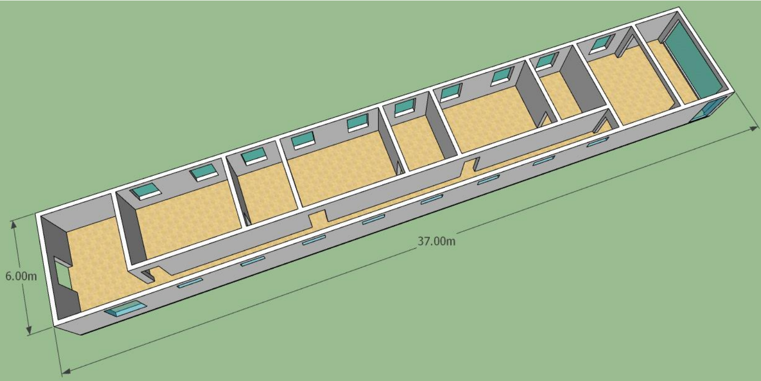
Figure 3-8: Living House
