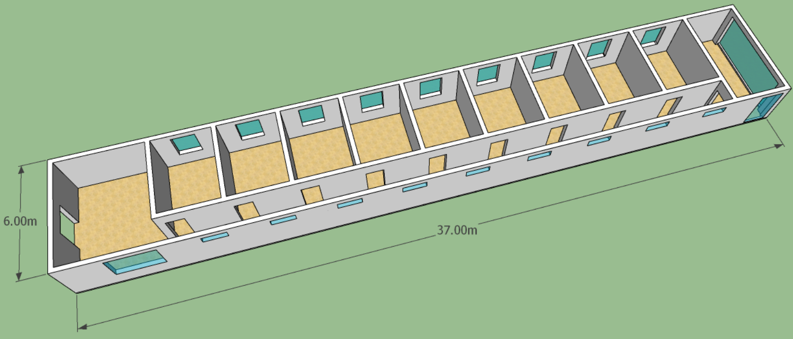
Figure 3-9: Living House
