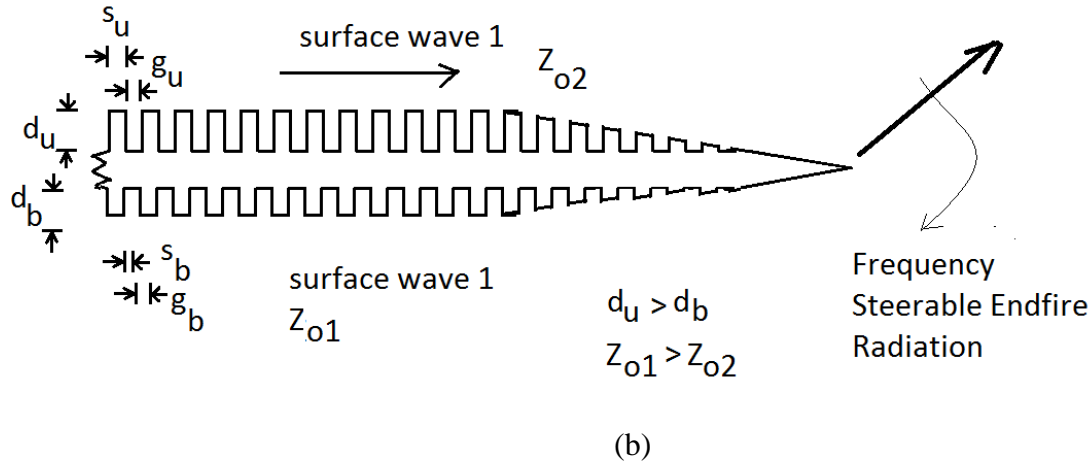
Figure 5. Mechanism of frequency dependent steering of endfire radiation. a) antenna no frequency steerable endfire radiation; b) antenna with frequency steerable endfire radiation.
