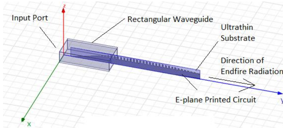
Figure 1. Basic version of the proposed E-plane endfire antenna.
