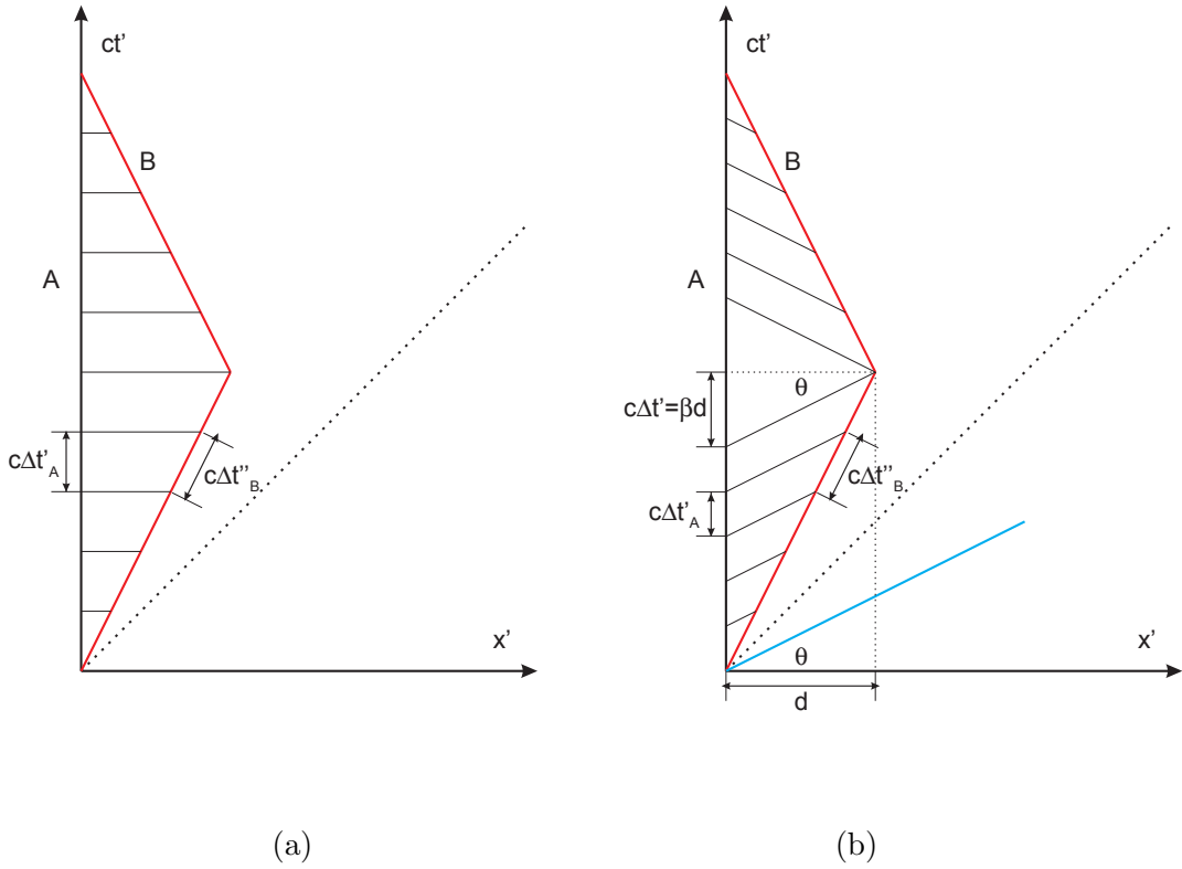
FIG. 1: Minkowski diagram for the twin paradox from Andrew's point of view (a) and from Bob's point of view (b).
