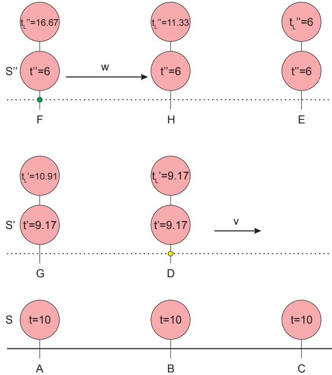
FIG. 3: ... at t = 10 ms Bob “jumps” to the moving frame S'' , to the position of clock F , in order to catch up Andrew; ...
