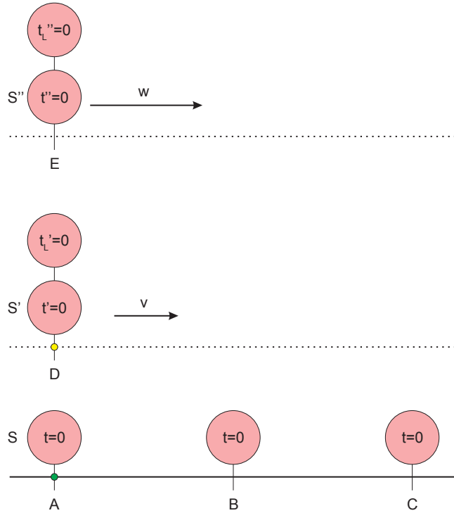
FIG. 2: All times in the figures are expressed in milliseconds and rounded to two decimal places. Twins Andrew and Bob, initially in the moving frame S' , separate at t = 0 ; Andrew (yellow dot) remains in frame S' with clock D , while Bob (green dot) “jumps” to the rest system S to the location of clock A ; ...
