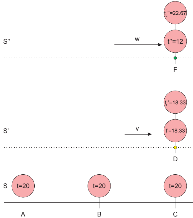
FIG. 4: ... the two twins meet again at t = 20 ms. Bob is younger.
