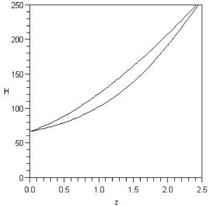
Figure 3. Dependence of the Hubble parameter ( \text{km} \cdot \text{sec}^{-1} \cdot \text{Mpc}^{-1} ) on red shift. The upper curve - \Lambda\text{CDM} -model, the lower curve – this theory.
