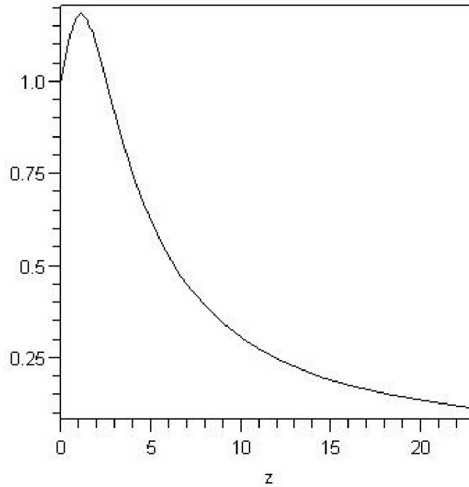
Figure 4. Dependence of the ratio of the Hubble parameter in \Lambda\text{CDM} -model to its value in this theory.
