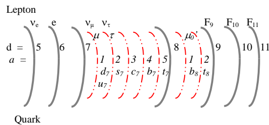
Figure 3. Leptons and quarks in the seven principal dimensional orbitals (solid lines) denoted by the principal dimensional orbital number d and the seven auxiliary dimensional orbitals (dash-dotted lines) denoted by the auxiliary dimensional number a .
