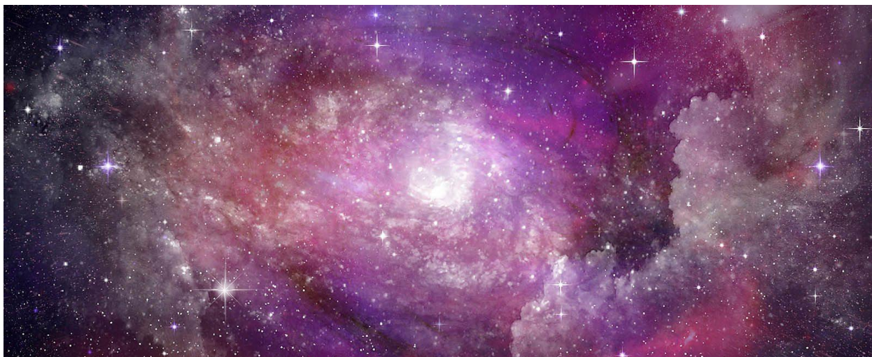
Fig. 1. Red luminescence of the Universe
