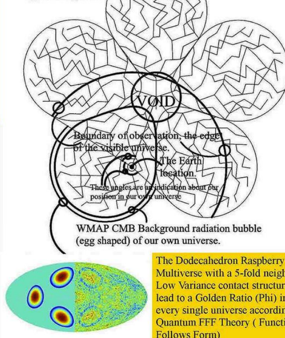
Figure 5, wavefunction collapse between CP symmetric mirror particles by instant entanglement between multi universal bubbles located around the Big Bang central void.
