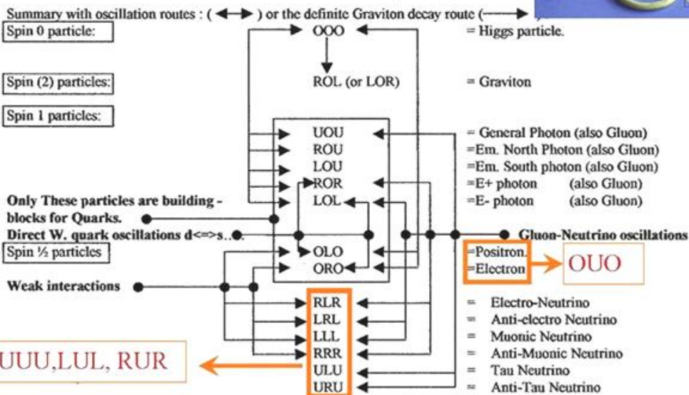
Figure 6. Alternative Feynman diagrams for di-monopole repeller forces. 5x monopole photons are also Gluons active for the Strong Force.
