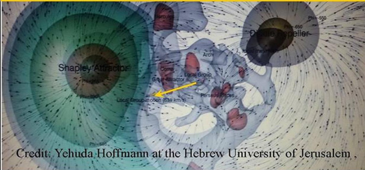
Credit: Yehuda Hoffmann at the Hebrew University of Jerusalem , Quantum Gravity as pressure distribution of the oscillating dual Higgs/Graviton vector field. New Dark Matter Black Hole, "Eat" the chiral oscillating Higgs vacuum.(Quantum-FFF Theory)
