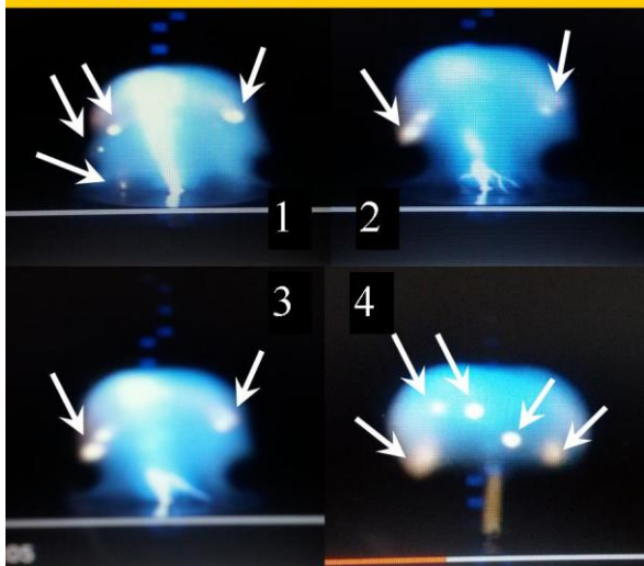
Figure 5, Microscopic unstable Black Holes accelerated by plasma tails on Earth: Ball lightning and micro comets
