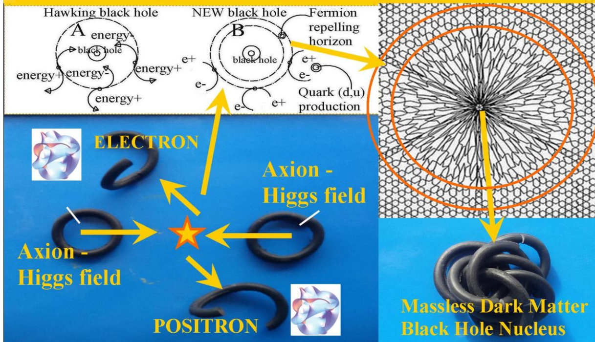
Figure 1, Pair production by Axion Higgs field collision at black hole horizons.
