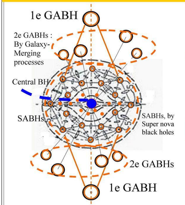
Figure 2. Dual external black hole configuration for dead galaxies without extra merger dark matter GABHs compared with more complex merger spiral galaxies with 1e and 2e GABHs (Galaxy Anchor Black Holes).
