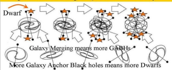
Figure 6. Dual Dark matter black holes of different sizes combined after galaxy merger processes.
