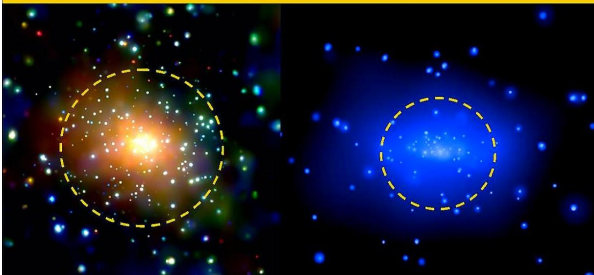
Figure 3. Black hole hierarchy through the cross section of galaxies.
