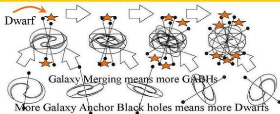
Figure 2. Dual external black hole configuration for dead galaxies without extra merger dark matter GABHs compared with more complex merger spiral galaxies with 1e and 2e GABHs (Galaxy Anchor Black Holes).
