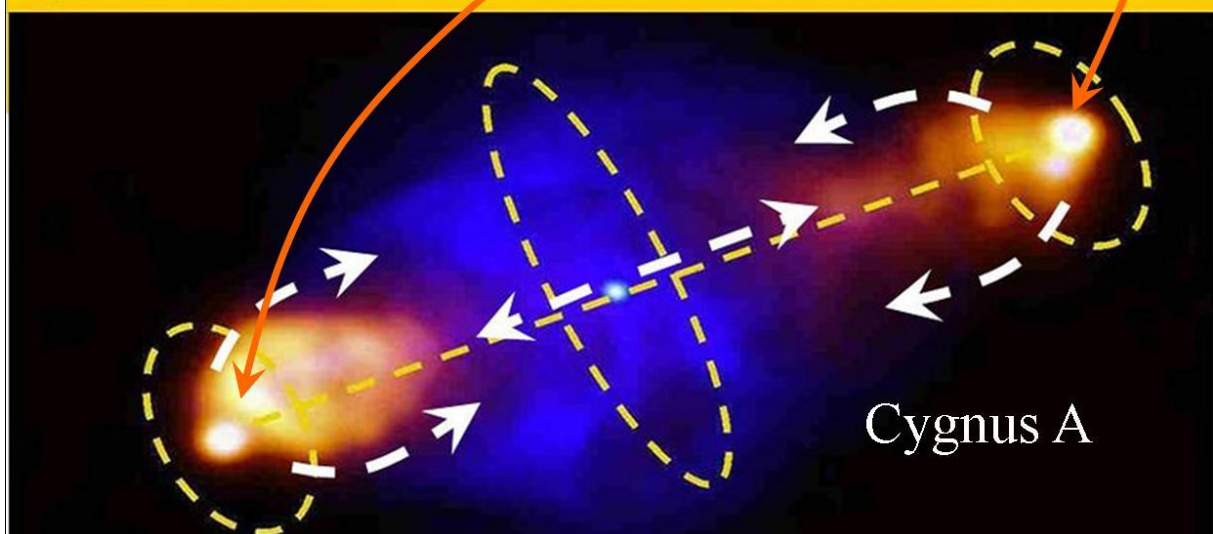
Figure 61, Markian 231 as rhe infant stage of Cygnus A. by By EDM Black Holes.
