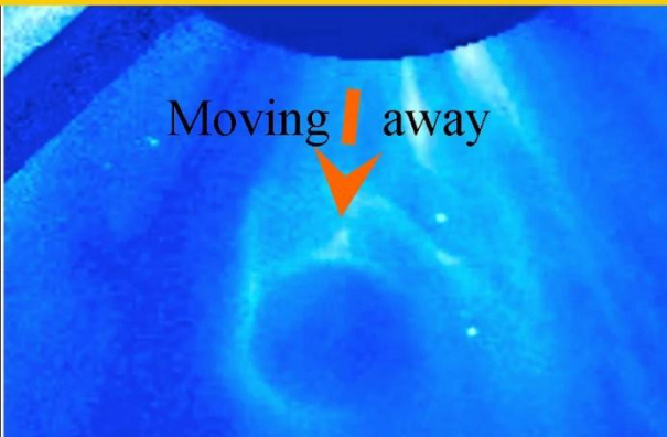
Figure 7, Even the sun seems to have polar dual black hole Herbig Haro remnants.
