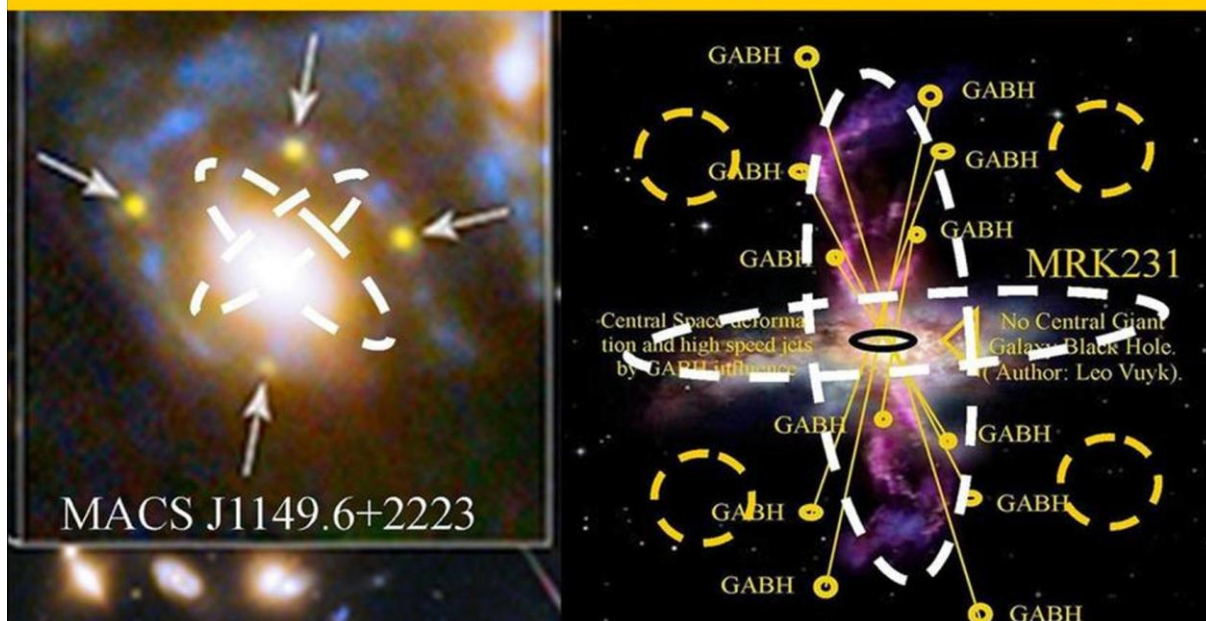
Figure 1. Einstein Cross effect originated by the Quadrupole shaped Dark Matter distribution of edge-on (merging?) Spiral Galaxies, like MACS J1149.6. Also MRK 231 seem to have a quadrupole dark matter distribution (according to Quantum FFF Theory).
