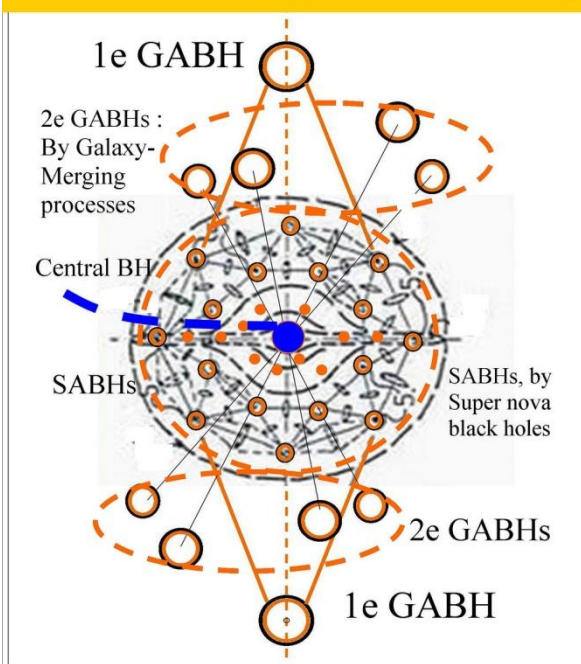
Figure 6. Dual Dark matter black holes of different sizes combined after galaxy merger processes.
