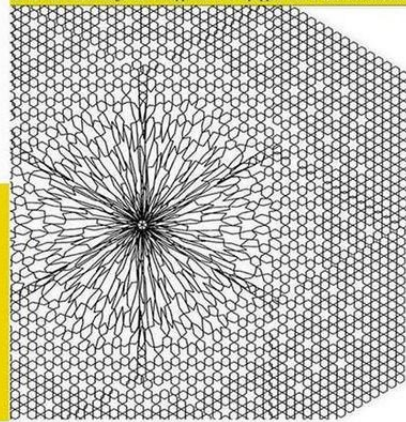
Figure 27, Quantum dimonopole repeller gravity ( the oscillating Casimir vacuum ) combined with less pressure from pushing gravitons.
