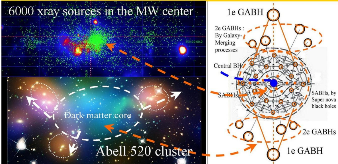
Figure 1, Merger dynamics of NON inertial Dark Matter black holes left behind after merging in the middle.
