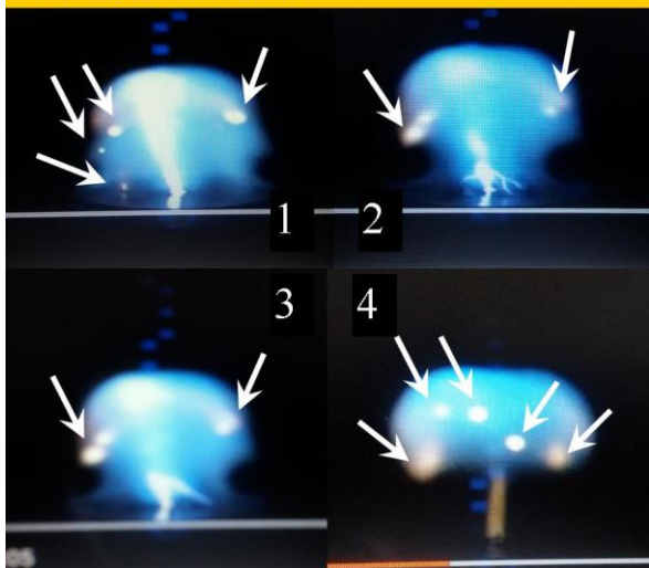
Figure 2, Microscopic Black Holes on Earth.
