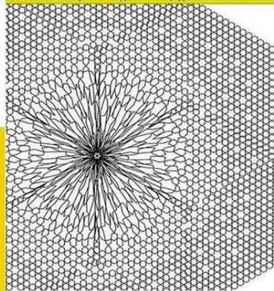
Figure 24, Quantum dipole repeller gravity ( the oscillating Casimir vacuum ) combined with less pressure from pushing gravitons.
