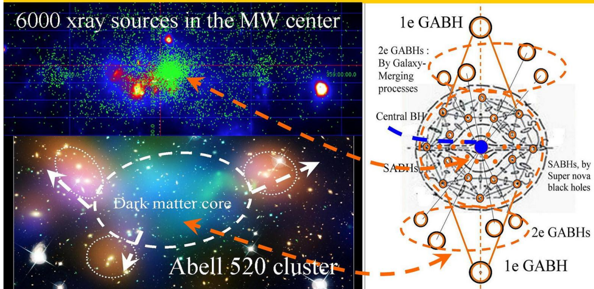
Figure 0, Merger dynamics of inertial Dark Matte black holes left behind after merging in the middle.
