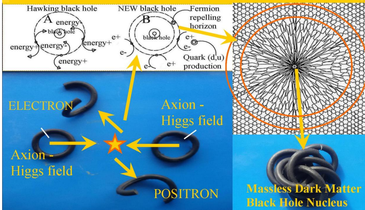
Figure 1. Pair production by Axion Higgs Field particle collision at black hole horizons (Q-FFF Theory)
