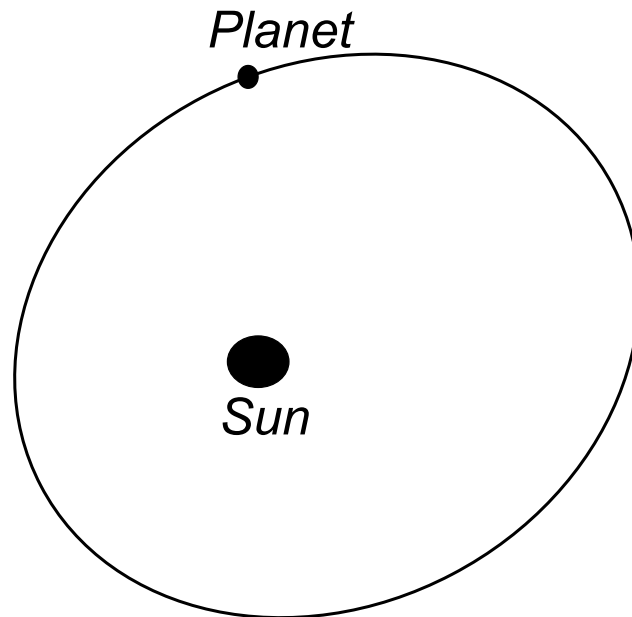
Heliocentric model
