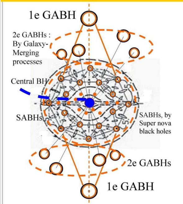
Figure 7. Dual Dark matter black holes of different sizes combined after galaxy merger processes.
