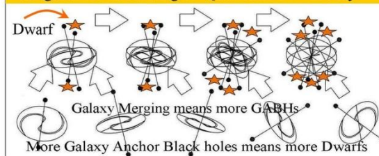
Figure 7. Dual Dark matter black holes of different sizes combined after galaxy merger processes.
