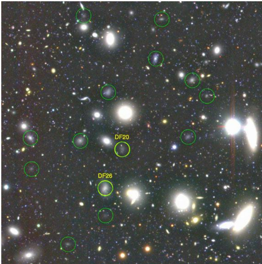
Figure 2. The Coma cluster with multiple Ultra Diffuse Galaxies ( encircled)
