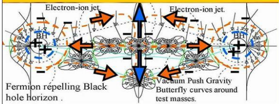
Cygnus A with dual plasma/gas producing "New physics" negative charged BHs as hotspots, with growing merger (SN) black hole in the center. Below: local Quantum vacuum push gravity vector butterflies originated by the BH vacuum absorption of dark vacuum energy.
