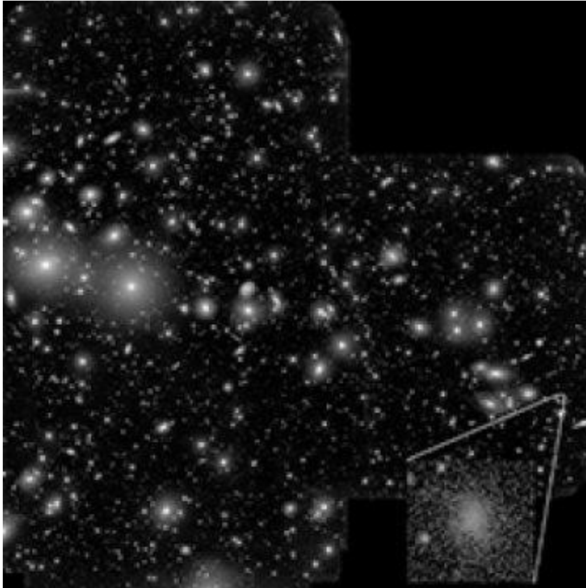
Figure 1, The Parseus cluster with enlarged one Ultra diffuse Galaxy.
