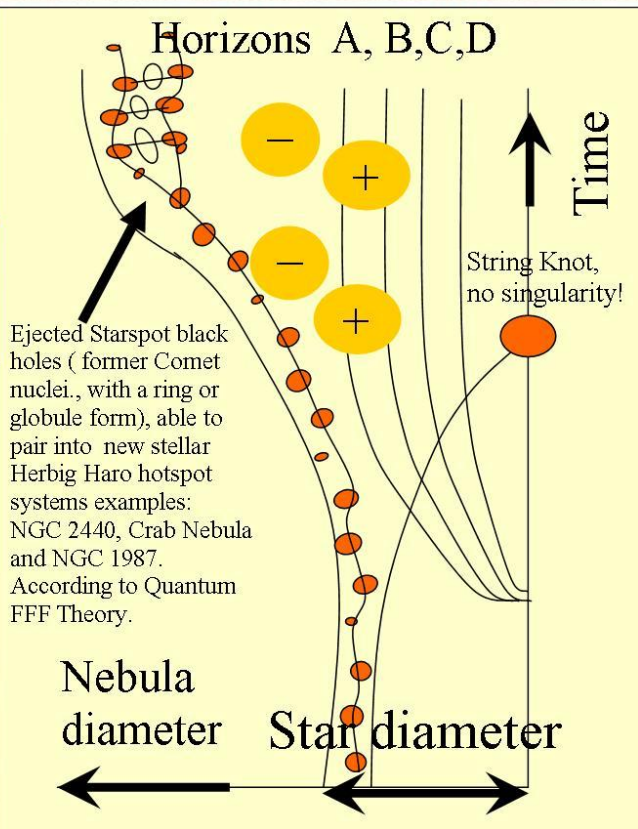
Figure 13, 4 different black hole horizons and the proliferation of small starspot black holes.
