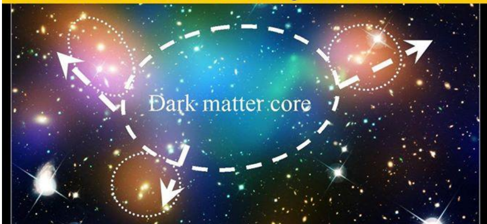
Figure 5, Dark matter peaks inside a large galaxy cluster, seem to represent the largest primordial GABHs ( Galaxy Anchor Black Holes) or Big Bang splinters. The peaks are additional to the “mountain of dark matter black holes” (Dark Matter Core) of all sizes down to Sunspot black holes, Comet nuclei and ball lightning.
