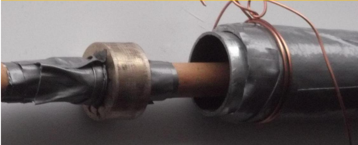
Figure 3. detail of the tube with composite circular magnet able to central magnetization of the tube.
