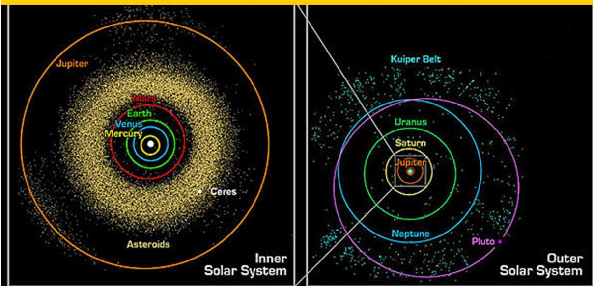
Figure: 18, The solar baby comets are supposed to travel onto the different clouds or belts like the Oort cloud and Kuiper- and Inner Jupiter belt.
